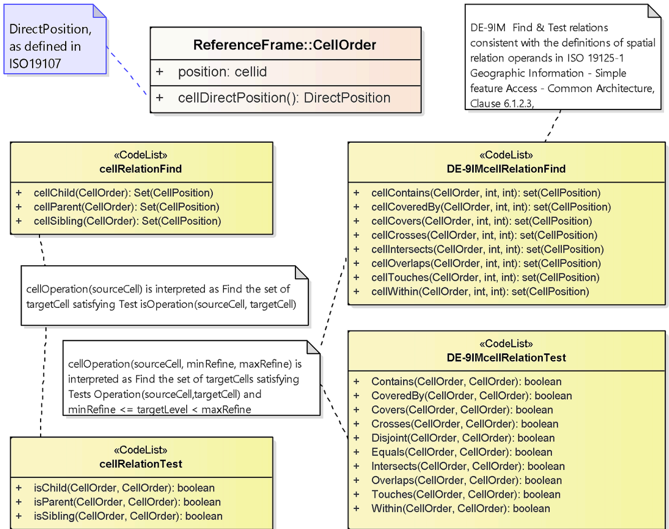
Figure 10 – DGGs Algebraic Operations functional algorithms class diagram
