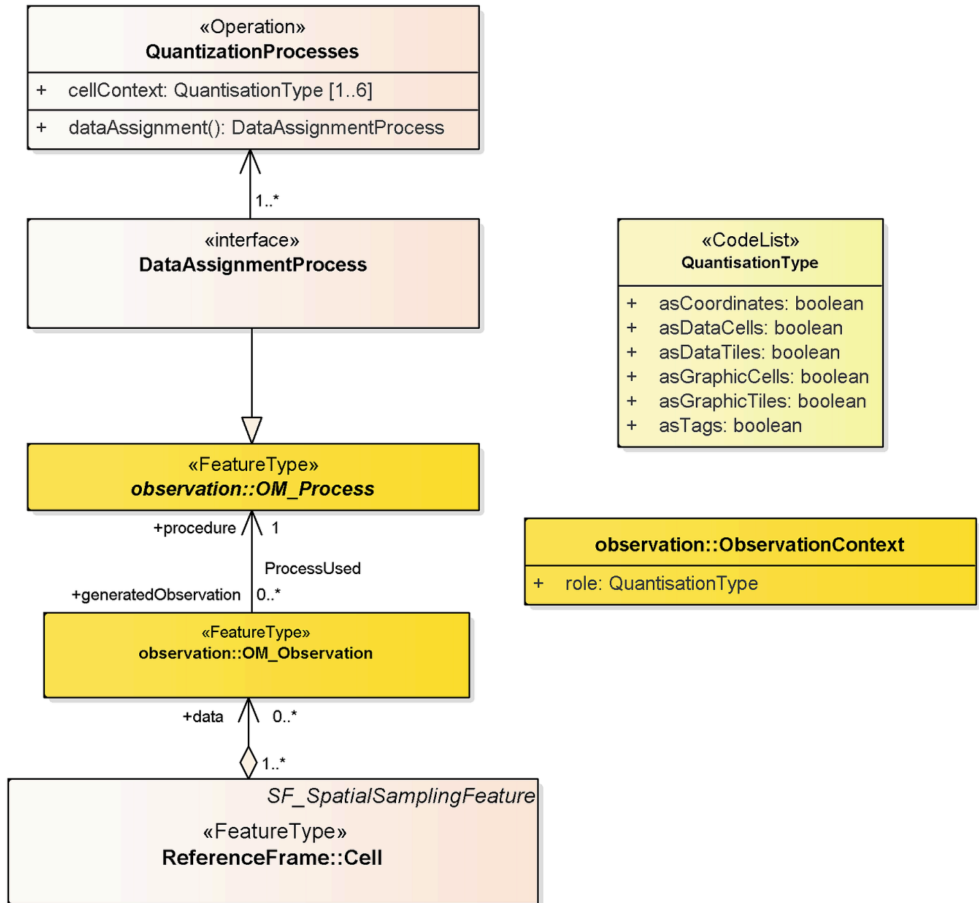
Figure 9 – DGGS Quantization functional algorithm class diagram
