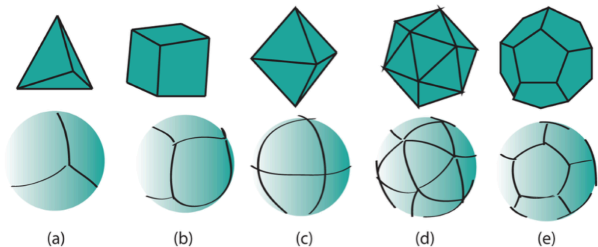
Figure 1 — Regular polyhedra (top) and their corresponding initial equal area tessellation (bottom) (a) tetrahedron, (b) cube, (c) octahedron, (d) icosahedron and (e) dodecahedron. [111111, Figure 2]
