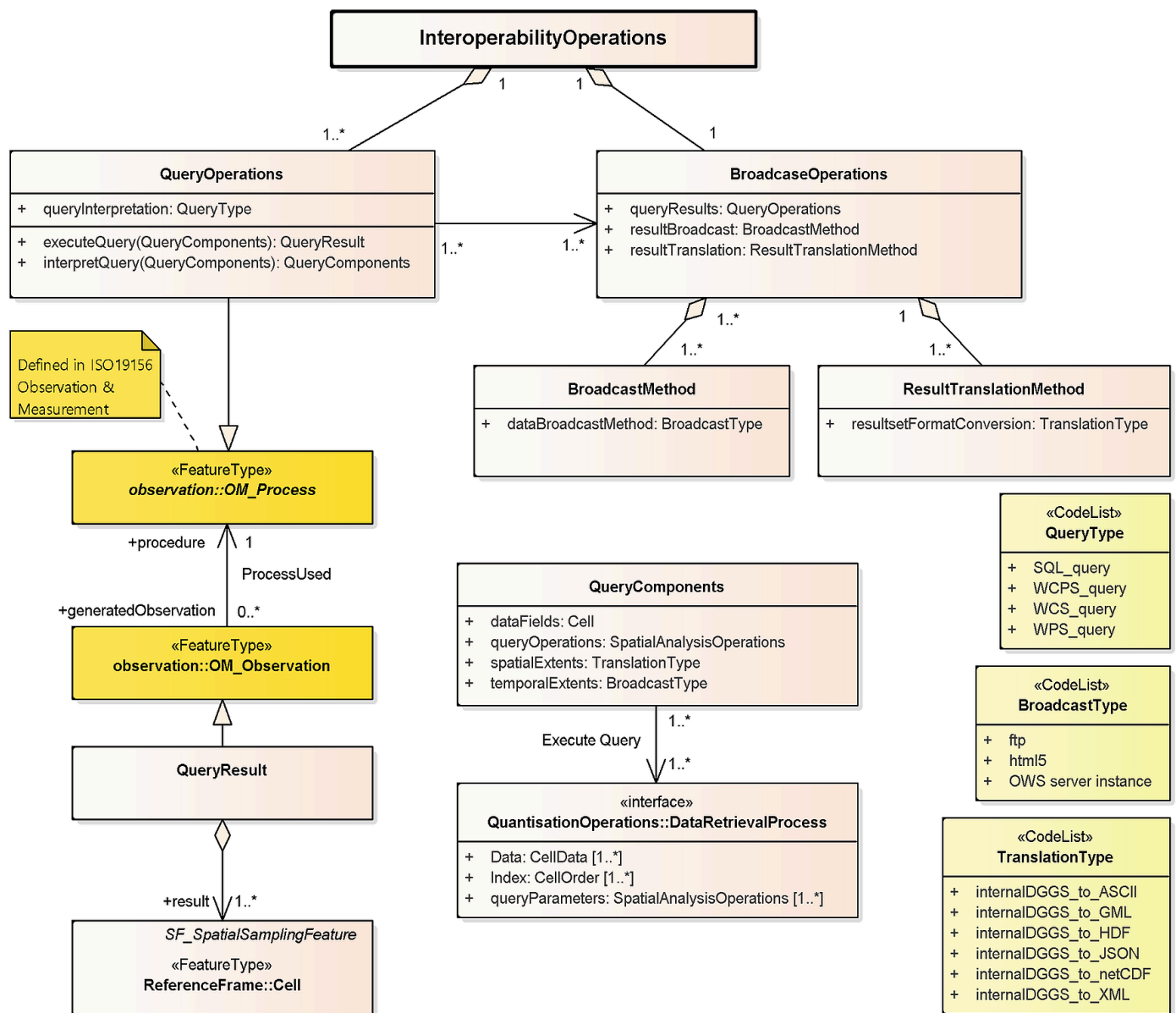
Figure 11 – DGGS Interoperability Operations functional algorithm class diagram
