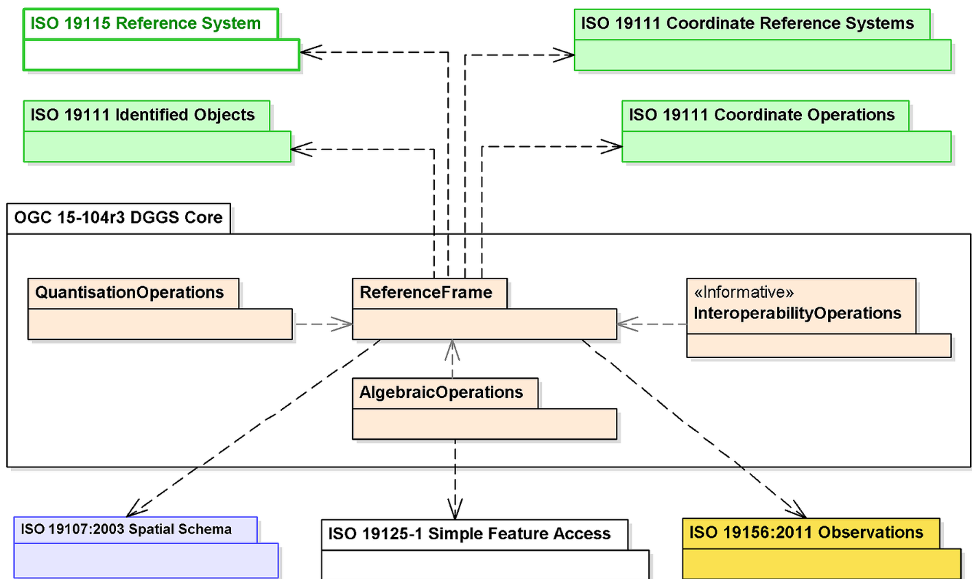
Figure 7 – DGGs Core Conceptual Data Model
