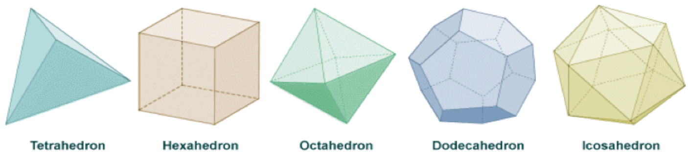
Figure B.2 – Representation of the five (5) Platonic solids: Tetrahedron, Hexahedron/Cube, Octahedron, Dodecahedron and Icosahedron.
