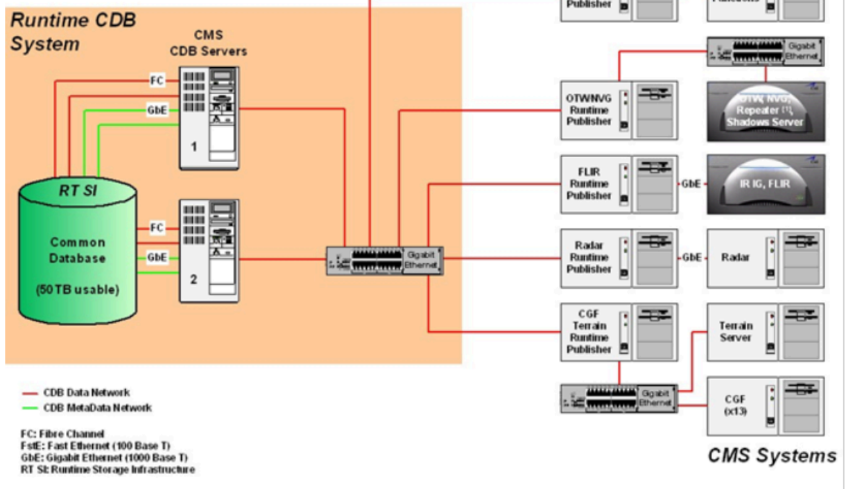
Figure 4 – Typical Implementation of CDB Standard on High-end Simulator
