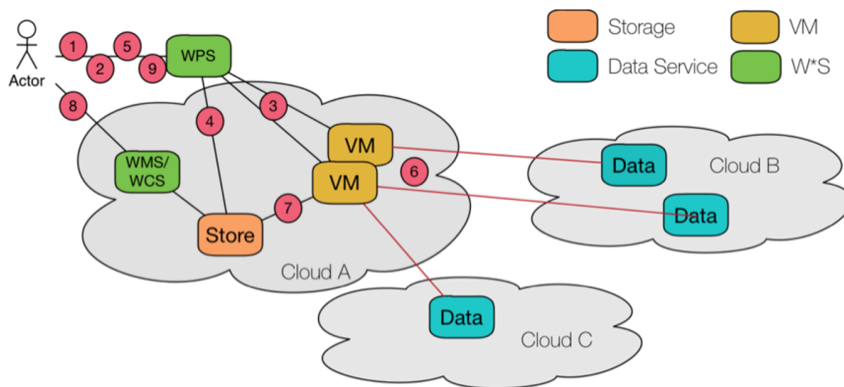
Figure 11 — OGC Testbed 13 Cloud Environment Overview
