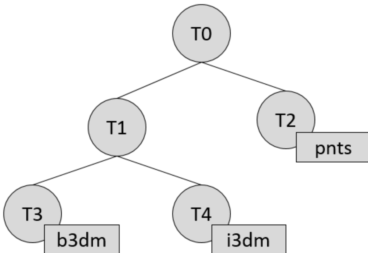
Figure 12 — A tileset with transformed children tiles
