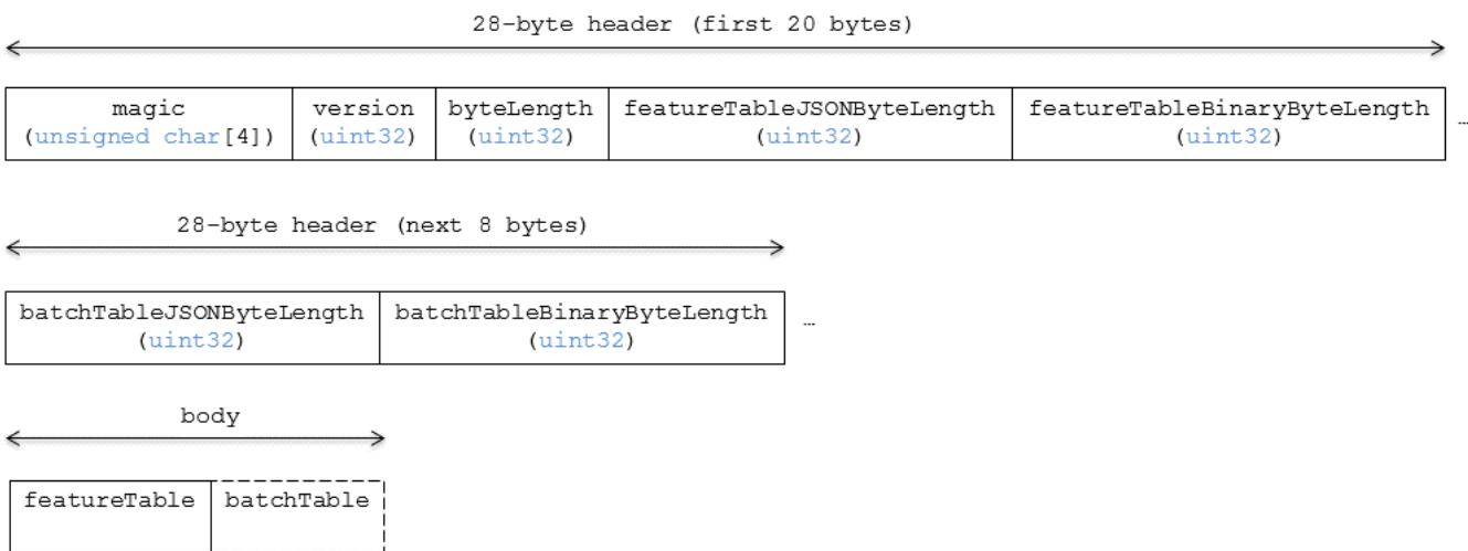
Figure 29 — Point Cloud layout
