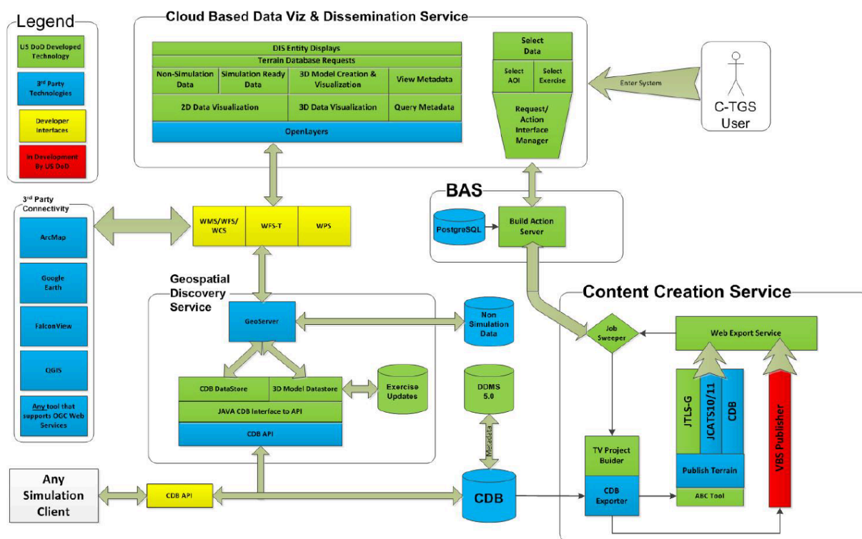
Figure 1 — DoD C-TGS Architecture (Chambers and Sherman, 2014)
