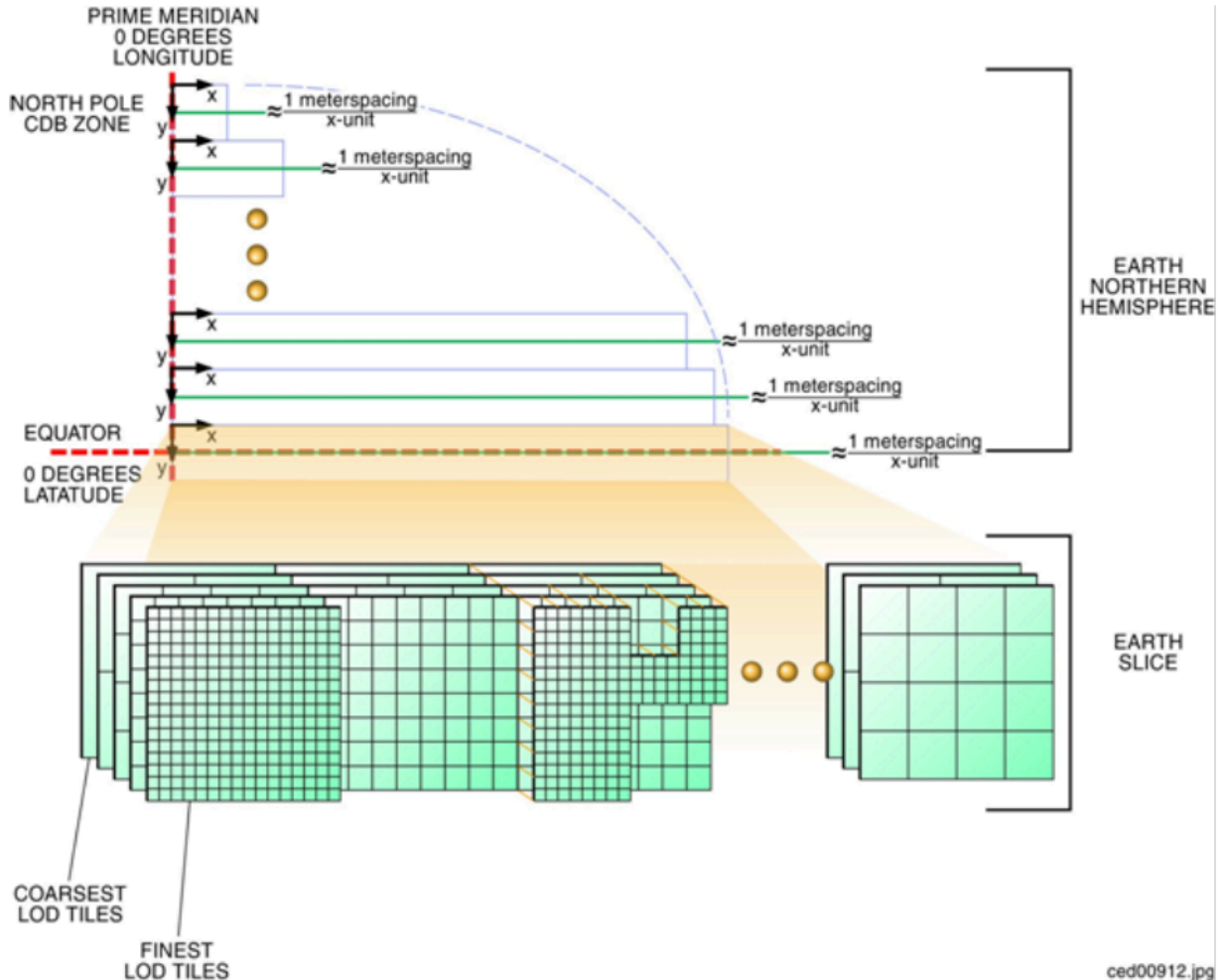
Figure 8 – Variable Allocation of LOD
