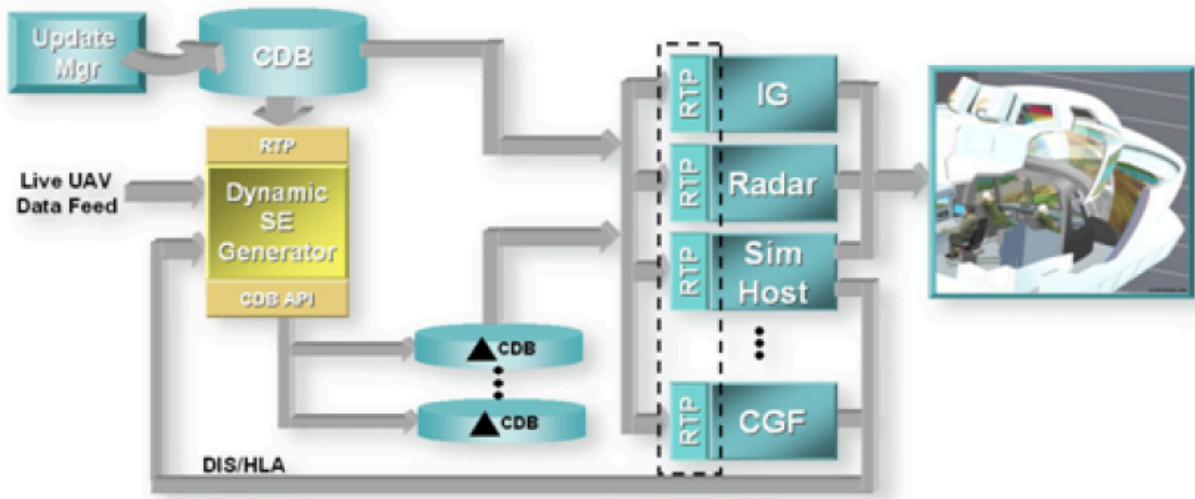
Figure 9 — Versioning Paradigm Applied to Dynamic SE
