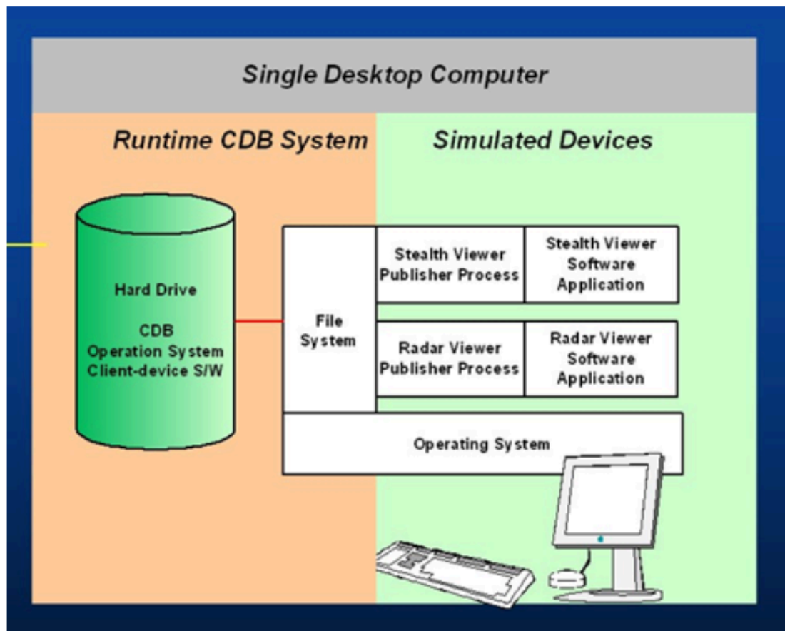
Figure 5 — Typical Implementation of CDB Standard on Desktop Computer
