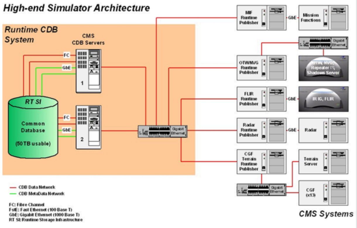
Figure 4 – Typical Implementation of CDB Standard on High-end Simulator
