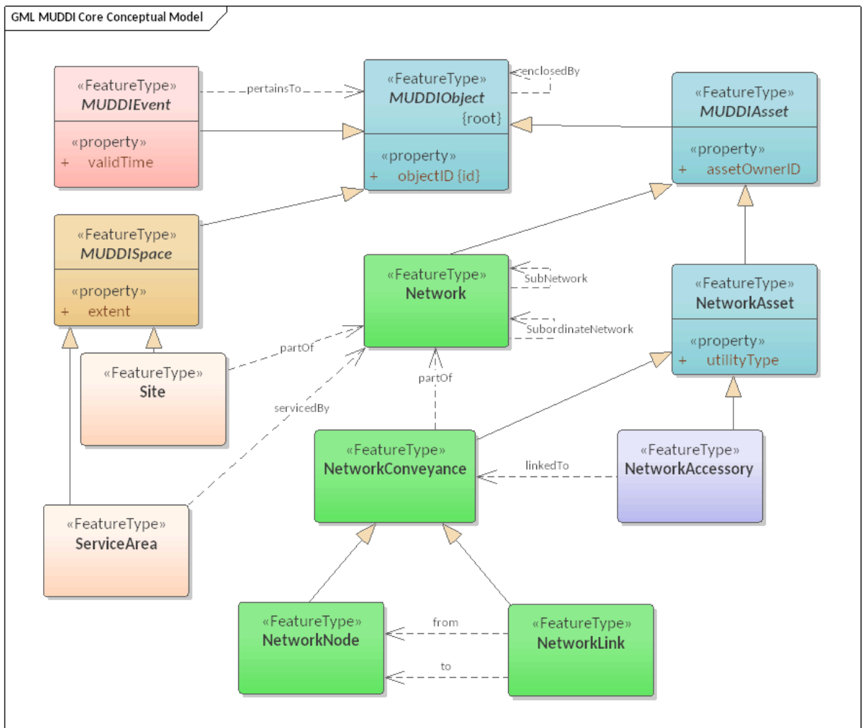
Figure 39-2 – EA-generated PNG file with correct layout
