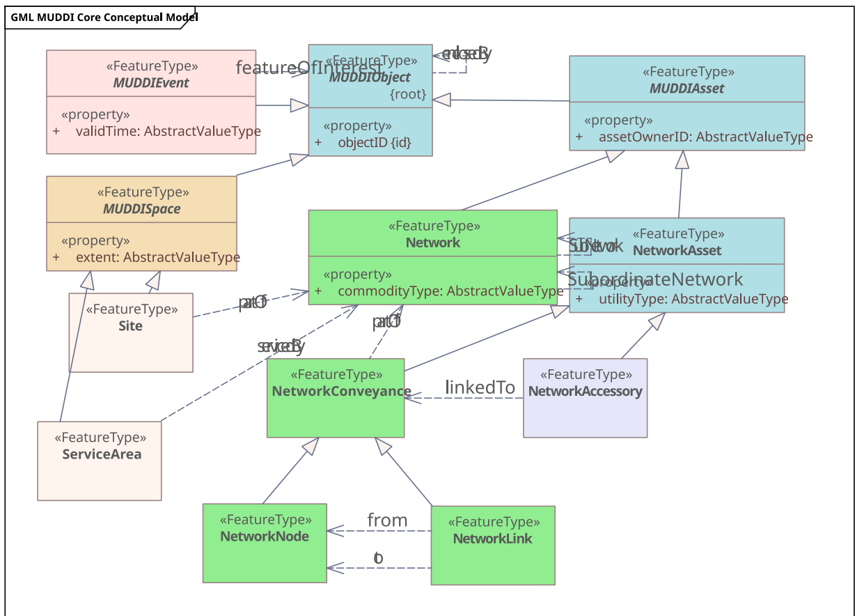
Figure 39-1 — EA-generated SVG file containing inaccurate layout
