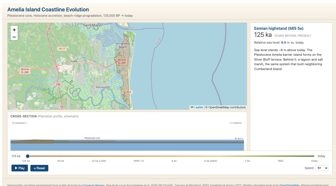
Figure 1: Eemian highstand, 125 ka. The Pleistocene core (Silver Bluff terrace) is forming under a sea level \sim 6 m above today’s. The cross-section shows the future-Amelia footprint as a single body above the dashed sea-level line; everything seaward of it will form later.
