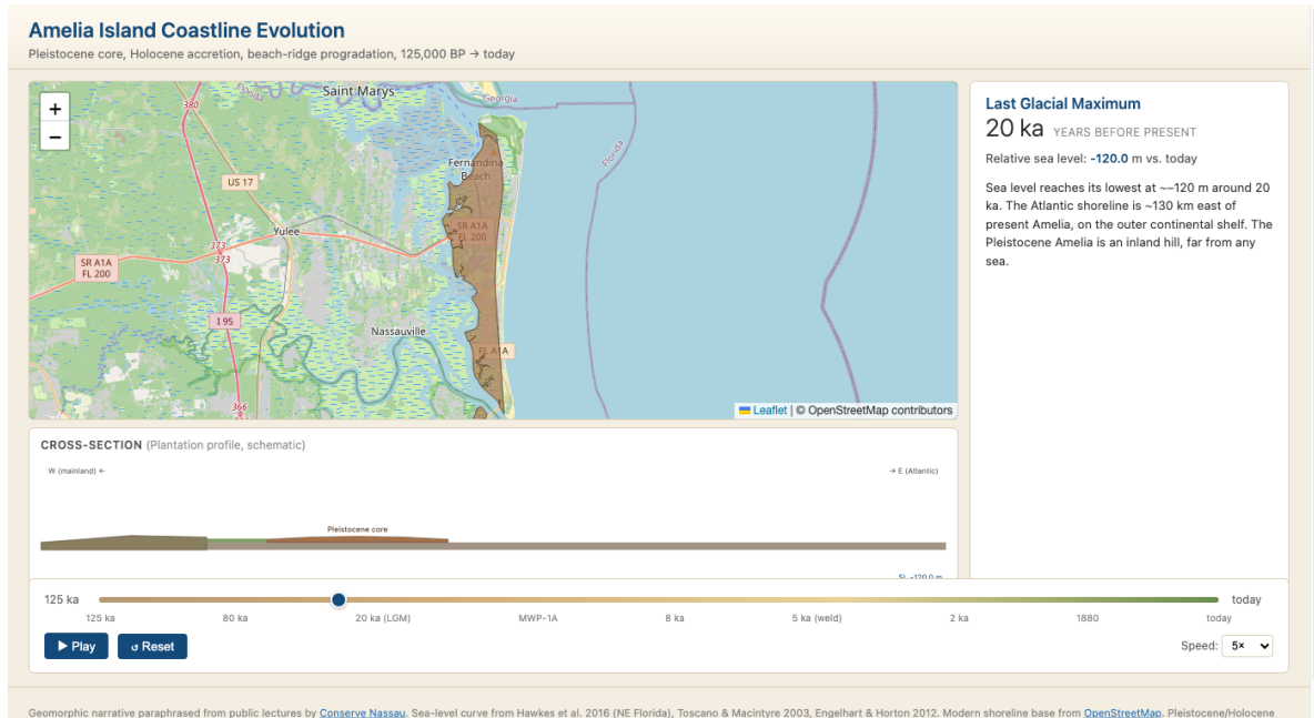
Figure 2: Last Glacial Maximum, 20 ka. Sea level -120 m. The red dashed hint line at the right edge of the map marks the LGM Atlantic shoreline \sim 130 km east. The Pleistocene Amelia stands as an inland hill, far from any coast.
