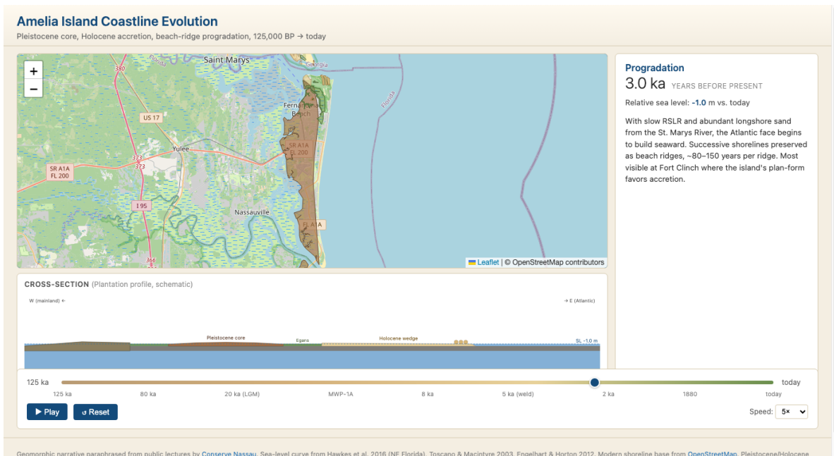
Figure 5: Mid-Holocene progradation, 3 ka. The Atlantic face begins building seaward. Beach ridges appear as small arcs near Fort Clinch (north end of the island). Sea level -1 m; sea-level rise has dropped well below the ~2 mm/yr stabilization threshold.
