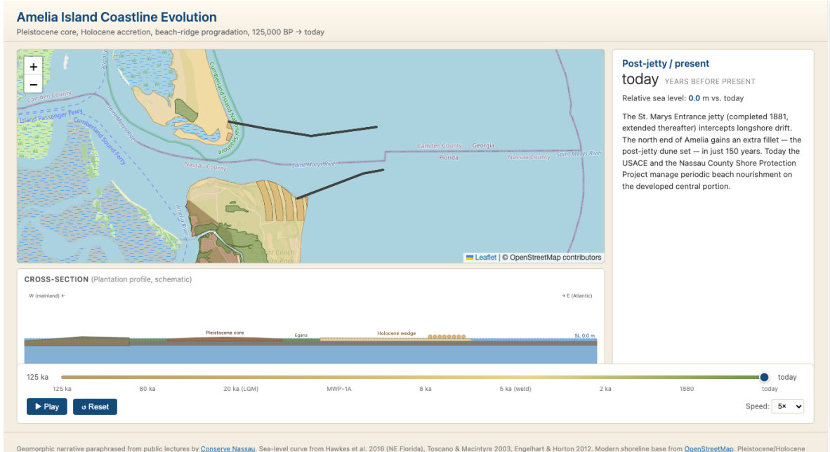
Figure 7: Zoomed view of the St. Marys River Entrance jetties at present-day (zoom 13). Both jetty geometries are pulled directly from NOAA Electronic Navigational Chart US5FL8CE (SLCONS layer, CATSLC=4). The North Jetty (upper line, Cumberland Island/Georgia side) is \sim 4.14 km long. The South Jetty (lower line, Amelia/Fort Clinch/Florida side) is \sim 2.50 km long. Both jetties were completed 1881–1893 by the US Army Corps of Engineers to maintain the navigation channel into Cumberland Sound. The ratio of approximately 1.65:1 (North:South) matches the surveyed geometry on the nautical chart.
