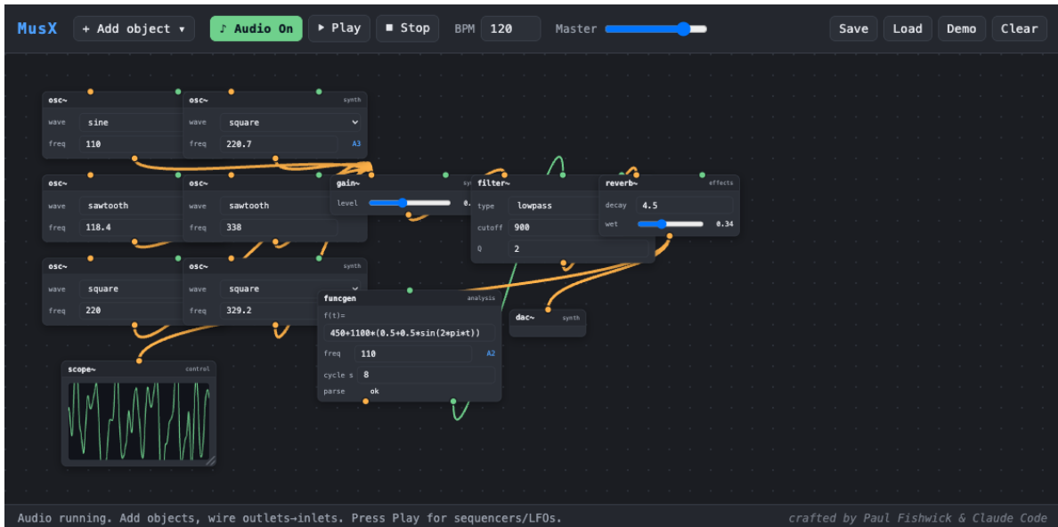
Figure 9: The “Layered Pad” demo (Max “Sound without limits”, patch 3): six detuned oscillators are mixed and passed through a filter whose cutoff is swept by a slow funcgen LFO, then reverberated. This emulates the MC (multichannel) oscillator bank of the original.
