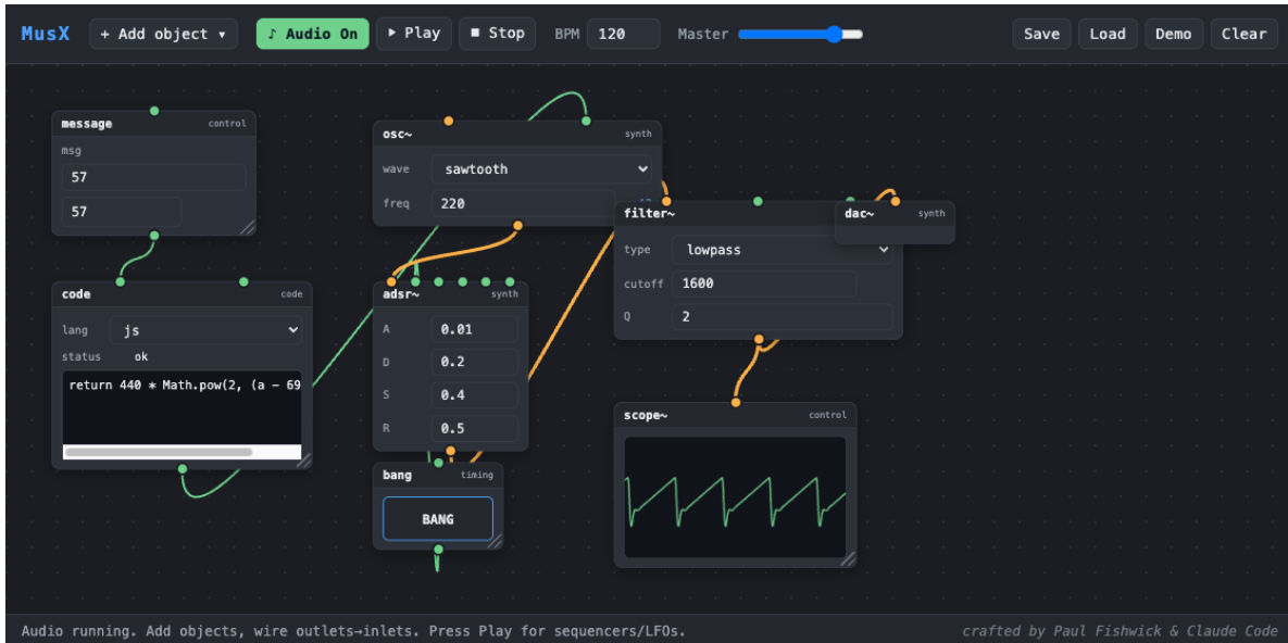
Figure 8: The “Bang + Code” patch. A message (MIDI 57) feeds a code object computing 440 * \text{Math.pow}(2, (a - 69) / 12) \rightarrow the oscillator’s frequency; the bang button triggers the adsr~ .
