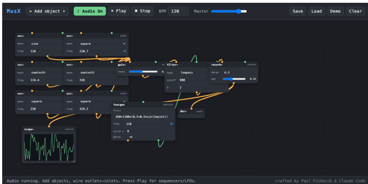
Figure 11: The “Layered Pad” demo (Max “Sound without limits”, patch 3): six detuned oscillators are mixed and passed through a filter whose cutoff is swept by a slow funcgen LFO, then reverberated. This emulates the MC (multichannel) oscillator bank of the original.
