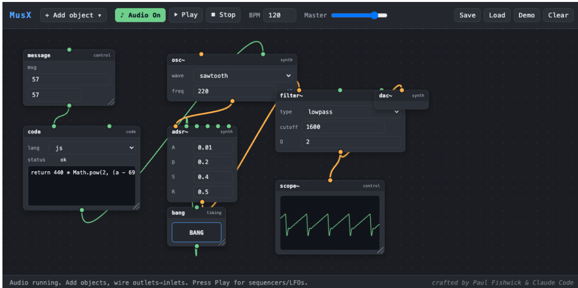
Figure 9: The “Bang + Code” patch. A message (MIDI 57) feeds a code object computing 440 * \text{Math.pow}(2, (a - 69) / 12) \rightarrow the oscillator’s frequency; the bang button triggers the adsr~ .
