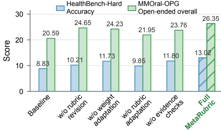
Figure 4: Component ablations. HealthBench-Hard accuracy-axis scores with Qwen3-4B and MMOral-OPG overall scores with Qwen3-VL-4B (0–100; ↑).
