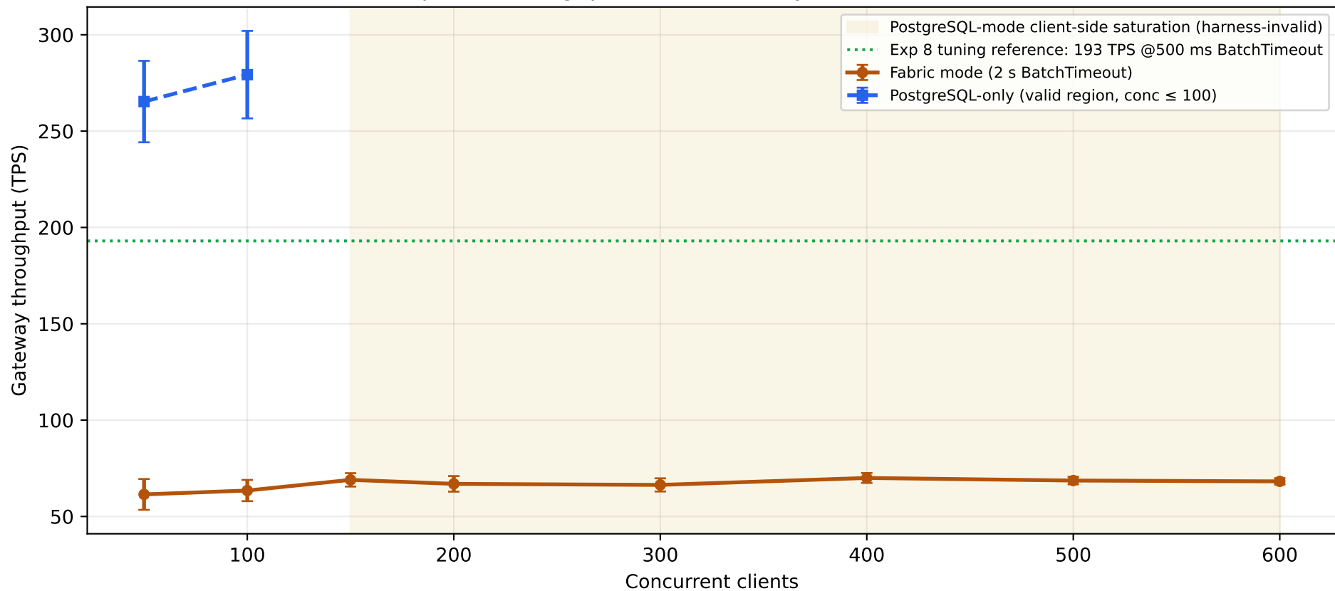
Exp 1 — Throughput vs concurrency, mean with 95% CI
