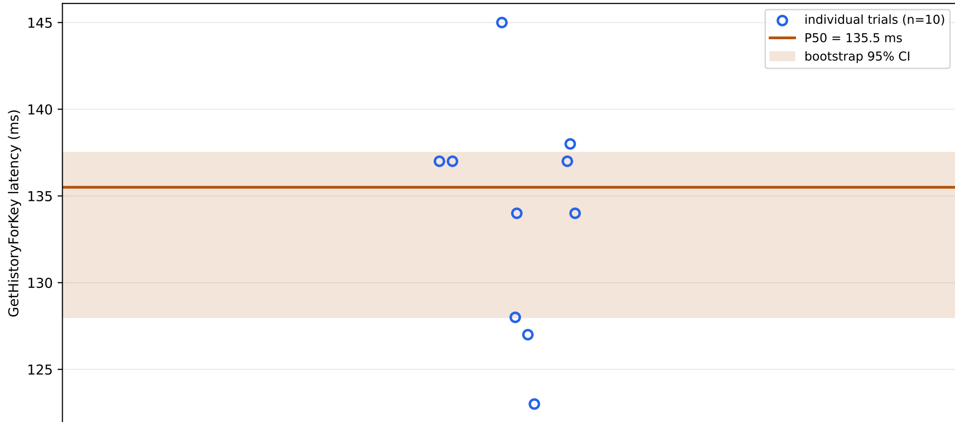
Exp 7 — Full-history query at depth 107 (peer CLI)
