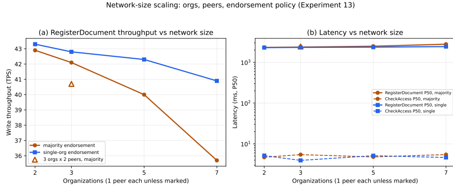
Figure 28: Experiment 13 network-size scaling across 2–7 organizations and endorsement policies: (a) write throughput; (b) write and read latency (log scale). Single-host deployment; inter-point ratios, not absolute TPS, are the meaningful result.
