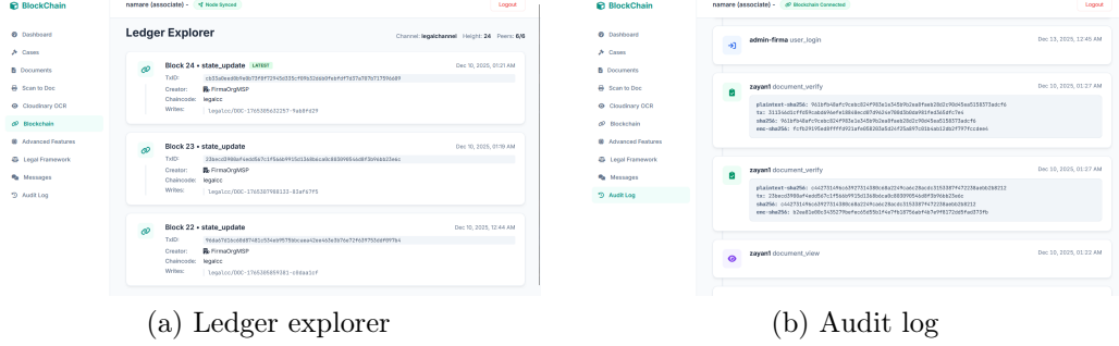
Figure 15: Audit and transparency views of the prototype interface.
