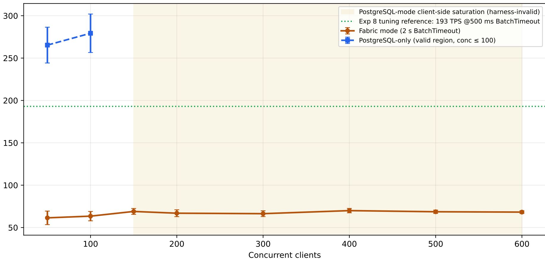
Gateway throughput (TPS)
