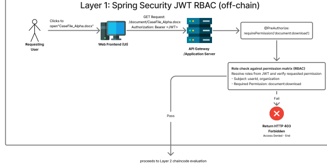
Figure 4: Layer 1 access control: Spring Security JWT RBAC at the API gateway. Requests failing role validation are rejected before reaching the blockchain layer.
