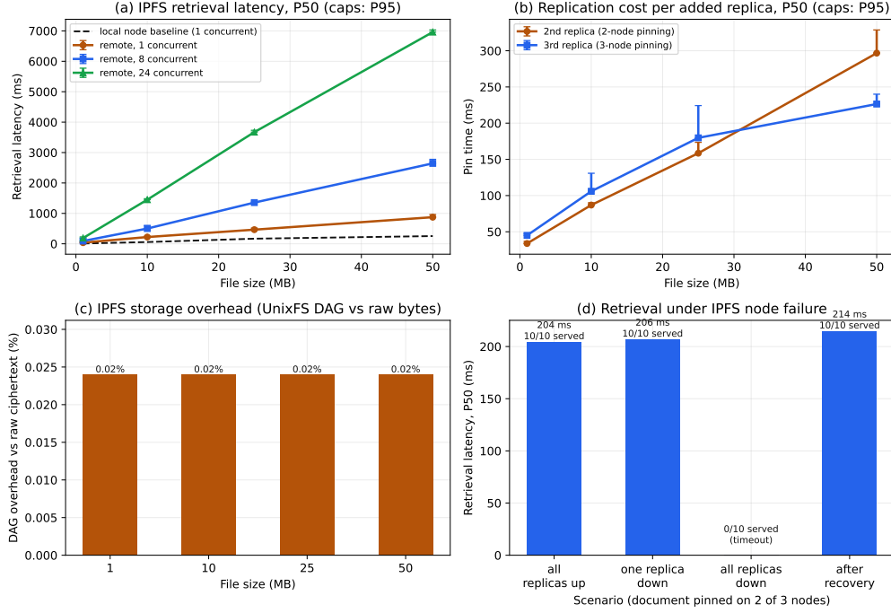
Figure 25: Experiment 10 IPFS storage/retrieval cost: (a) retrieval latency vs. file size and concurrency (local vs. cross-node); (b) replication cost per added replica; (c) constant 0.024 % UnixFS DAG overhead; (d) retrieval under node failure with a document pinned on 2 of 3 nodes.
