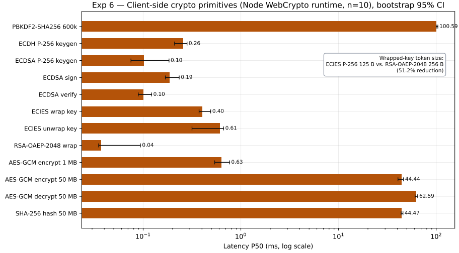
Figure 20: Experiment 6 cryptographic primitive benchmark using Node.js WebCrypto fallback (Linux; P50 with bootstrap 95% CIs, n=10 , log scale): PBKDF2-SHA256, ECDH/ECDSA operations, ECIES and RSA-OAEP key wrapping, AES-GCM, and SHA-256, with the wrapped-key token-size comparison (ECIES 125 B vs. RSA-OAEP-2048 256 B) annotated.
