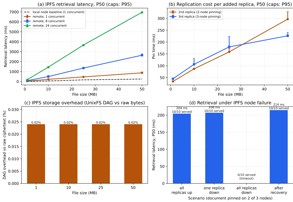
Figure 24: Experiment 10 IPFS storage/retrieval cost: (a) retrieval latency vs. file size and concurrency (local vs. cross-node); (b) replication cost per added replica; (c) constant 0.024% UnixFS DAG overhead; (d) retrieval under node failure with a document pinned on 2 of 3 nodes.
