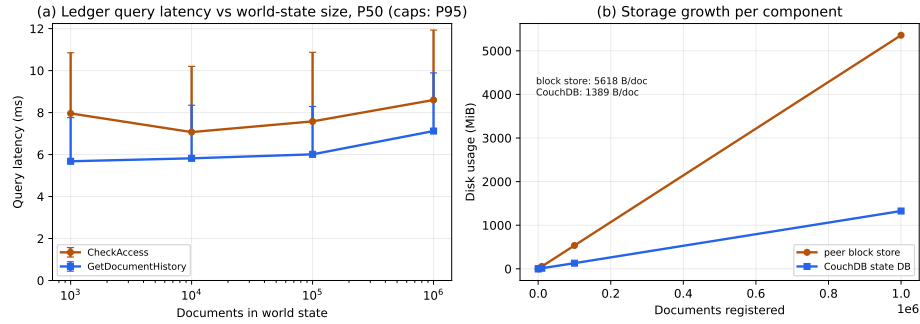
Figure 26: Experiment 12 ledger-growth scaling from 10 3 to 10 6 registered documents: (a) release-path query latency vs. world-state size (P50, caps P95); (b) linear per-peer storage growth ( \approx 7 KB/document across block store and CouchDB).
