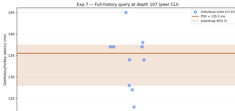
Figure 21: Experiment 7 Fabric GetHistoryForKey latency at the measured 107-entry history depth: all ten individual trials ( n=10 ) with the median (135.5 ms) and its bootstrap 95% confidence interval. Only measured data are shown; no extrapolation to deeper histories is plotted. Multi-depth validation is future work.
