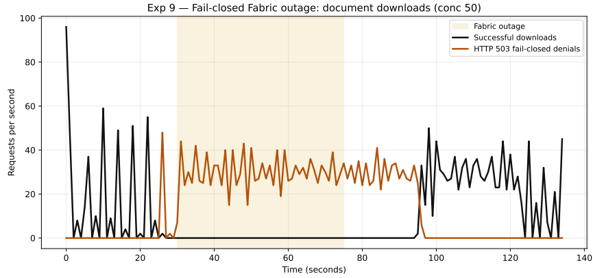
Figure 23: Experiment 9 fail-closed Fabric peer outage (computed from the released raw data): zero successful downloads during the 45s outage window; 1,340 HTTP 503 denial responses and 2,013 PostgreSQL audit rows (the difference reflects additional system-level audit events per denial). Denials visibly persist \approx 20 s past peer restart ( t = 75-95 s): the access-path circuit breaker completes its 30s open-state window before half-open probes readmit Fabric calls, after which normal operation resumes without intervention.
