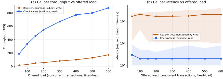
Figure 25: Experiment 11 Hyperledger Caliper benchmark of the deployed chaincode via the peer-gateway API: (a) throughput and (b) latency vs. offered fixed load for CheckAccess (evaluate) and RegisterDocument (submit). Caliper reports average/min/max latency, the convention used by comparable published systems.
