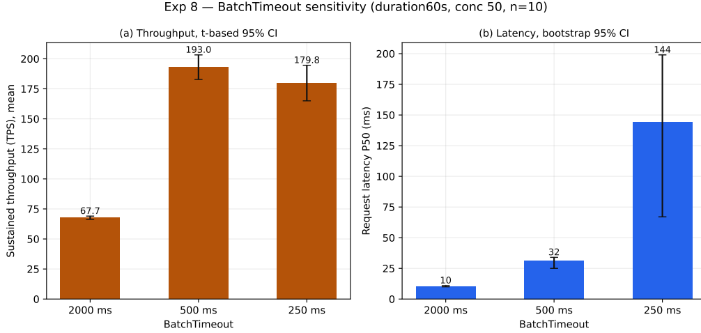
Figure 22: Experiment 8 BatchTimeout sensitivity (Linux x86_64, 50 clients; n=10 per setting, zero-error runs): (a) sustained throughput (mean, t 95 % CI) and (b) request latency (P50, bootstrap 95 % CI) at 2s, 500 ms, and 250 ms, showing the reproducible 500 ms optimum.
