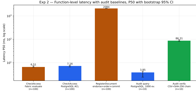
Figure 16: Experiment 2 function-level latency (P50, log scale; Linux, JVM-warmed; bootstrap 95 % confidence intervals): CheckAccess in both modes ( n=100 each, overlapping CIs), RegisterDocument ( n=100 ), and the Experiment 4 audit trust/latency baselines ( n=10 each).
