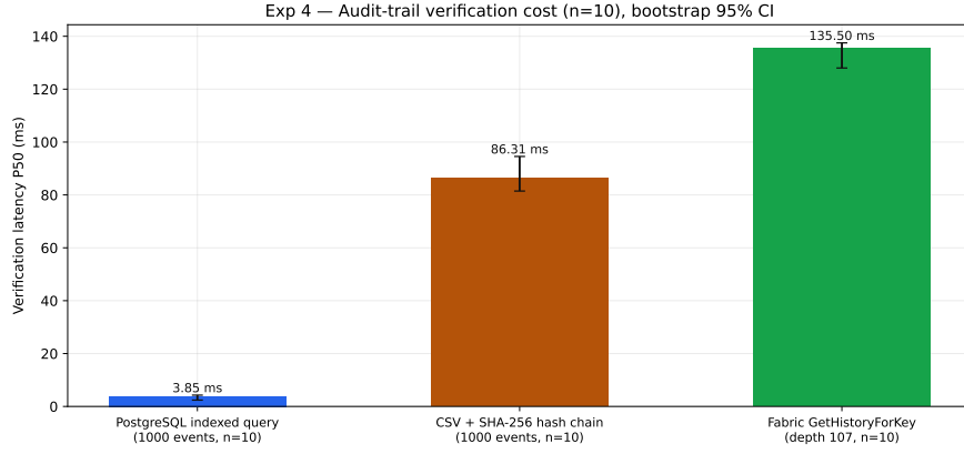
Figure 18: Experiment 4 audit verification efficiency (P50 with bootstrap 95 % CIs, n=10 each): PostgreSQL indexed queries, manual CSV + SHA-256 chain verification, and Fabric GetHistoryForKey ledger-verifiable history (depth 107, from Experiment 7).
