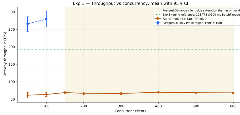
Figure 15: Experiment 1 scalability under concurrent load on Linux x86_64 (computed from the released raw data; mean with 95 % t confidence intervals, n=5 per point): Fabric REST-gateway throughput compared with the PostgreSQL-only baseline restricted to its harness-valid region ( \text{conc} \leq 100 ); the shaded region marks PostgreSQL-mode client-side load-generator saturation (self-flagged invalid rows, excluded from analysis), and the dotted line is the Experiment 8 BatchTimeout tuning reference (193 TPS at 500 ms).
