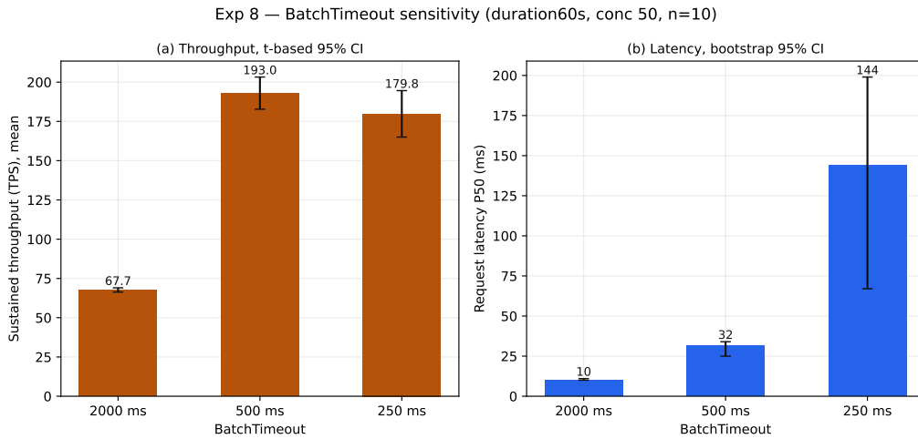
Figure 26: Experiment 8 BatchTimeout sensitivity (Linux x86_64 , 50 clients; regenerated, n=10 per setting, zero-error runs): (a) sustained throughput (mean, t 95 % CI) and (b) request latency (P50, bootstrap 95 % CI) at 2 s, 500 ms, and 250 ms, showing the reproducible 500 ms optimum.
