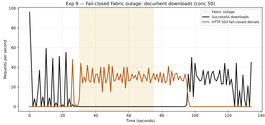
Figure 27: Experiment 9 fail-closed Fabric peer outage (computed from the released raw data): zero successful downloads during the 45 s outage window; 1,340 HTTP 503 denial responses and 2,013 PostgreSQL audit rows (the difference reflects additional system-level audit events per denial). Denials visibly persist \approx 20 s past peer restart ( t = 75\text{--}95 s): the access-path circuit breaker completes its 30 s open-state window before half-open probes readmit Fabric calls, after which normal operation resumes without intervention.
