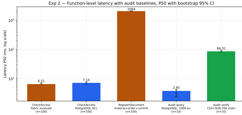
Figure 20: Experiment 2 function-level latency (P50, log scale; Linux, JVM-warmed; bootstrap 95 % confidence intervals): CheckAccess in both modes ( n=100 each, overlapping CIs), RegisterDocument ( n=100 ), and the Experiment 4 audit trust/latency baselines ( n=10 each).
