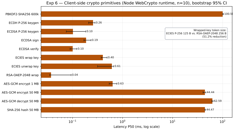
Figure 24: Experiment 6 cryptographic primitive benchmark using Node.js WebCrypto fallback (Linux; P50 with bootstrap 95% CIs, n=10 , log scale): PBKDF2-SHA256, ECDH/ECDSA operations, ECIES and RSA-OAEP key wrapping, AES-GCM, and SHA-256, with the wrapped-key token-size comparison (ECIES 125 B vs. RSA-OAEP-2048 256 B) annotated.
