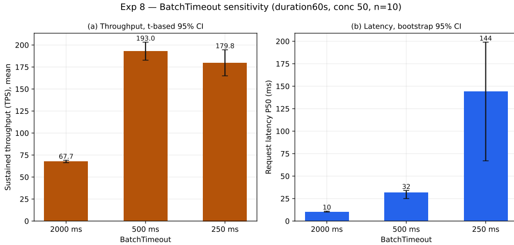
Figure 26: Experiment 8 BatchTimeout sensitivity (Linux x86_64, 50 clients; n=10 per setting, zero-error runs): (a) sustained throughput (mean, t 95 % CI) and (b) request latency (P50, bootstrap 95 % CI) at 2s, 500 ms, and 250 ms, showing the reproducible 500 ms optimum.
