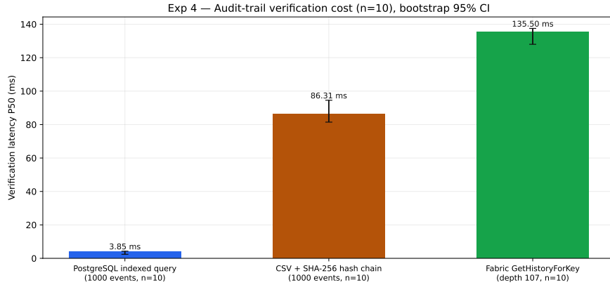
Figure 22: Experiment 4 audit verification efficiency (P50 with bootstrap 95 % CIs, n=10 each): PostgreSQL indexed queries, manual CSV + SHA-256 chain verification, and Fabric GetHistoryForKey ledger-verifiable history (depth 107, from Experiment 7).
