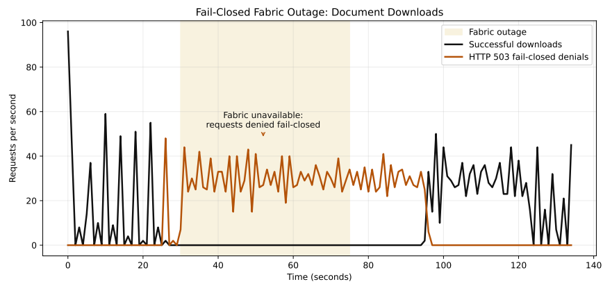
Figure 28: Experiment 9 fail-closed Fabric peer outage: zero successful downloads during the 45 s outage window; 1,340 HTTP 503 denial responses and 2,013 PostgreSQL audit rows (the difference reflects additional system-level audit events per denial); normal operation resumes after approximately 15 s gRPC reconnection lag.
