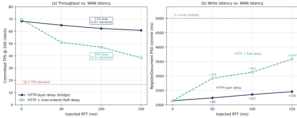
Figure 24: Experiment 5 WAN resilience (tc netem, Linux x86_64, 200 clients), comparing bridge-only and bridge + veth delay effects on TPS and RegisterDocument latency.
