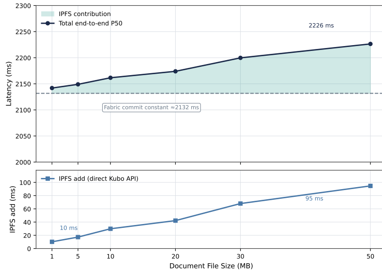
Figure 22: Experiment 3 file-size independence of ledger latency (Linux, direct Kubo API), separating server-side P50, IPFS upload range (10–95 ms), and constant Fabric commit latency.
