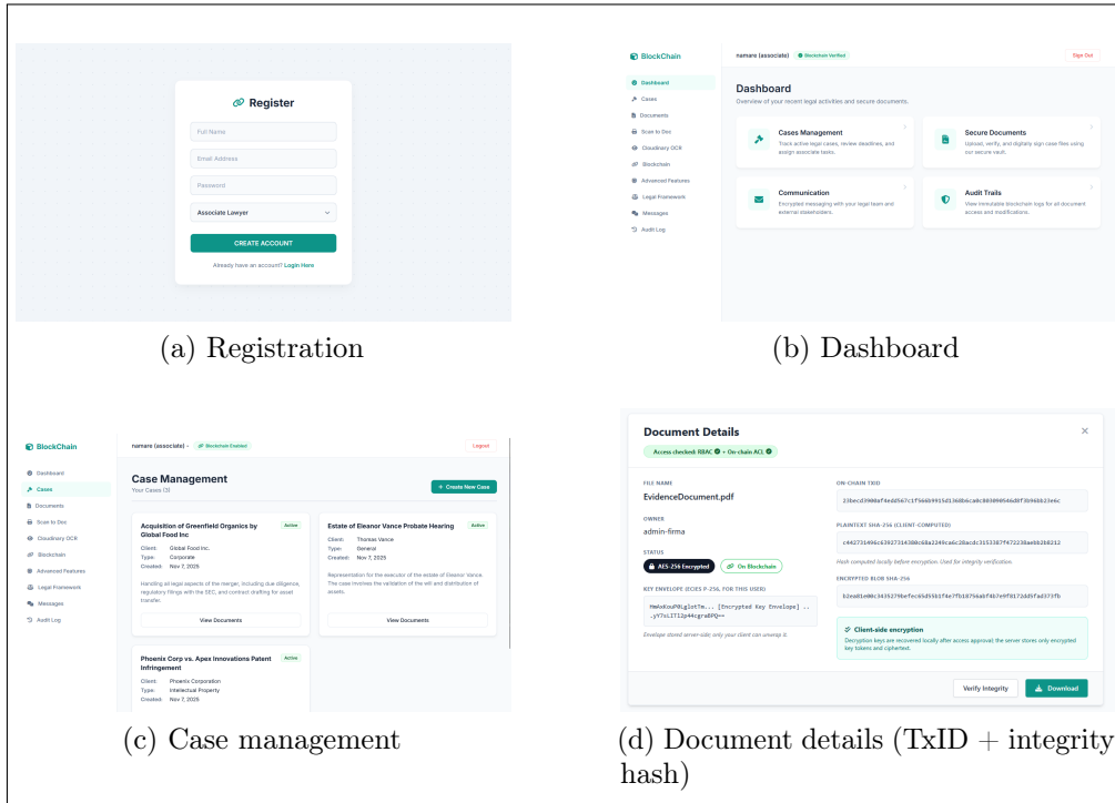
Figure 18: Prototype user interface.
