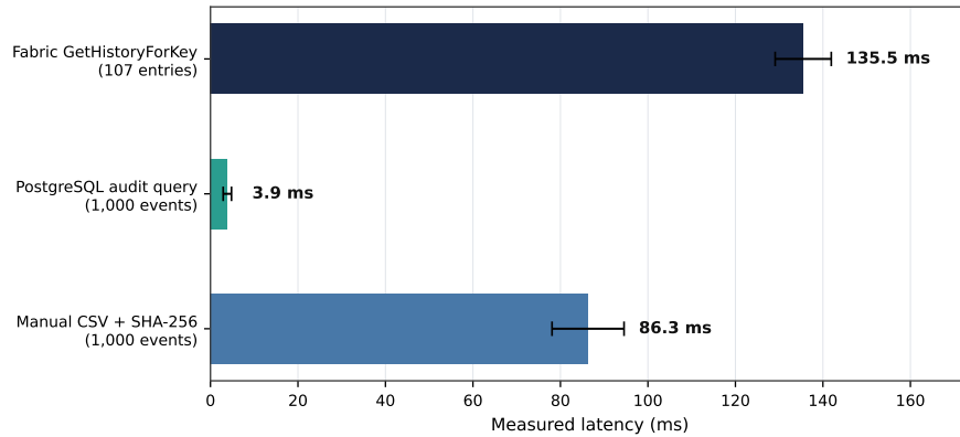
Figure 23: Experiment 4 audit verification efficiency across PostgreSQL queries, manual CSV + SHA-256 verification, and Fabric GetHistoryForKey ledger-verifiable history.
