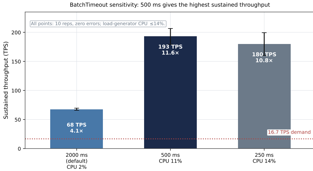
Figure 27: Experiment 8 BatchTimeout sensitivity (Linux x86_64, 50 clients), showing default 2s, 500 ms, and 250 ms throughput with zero-error runs.
