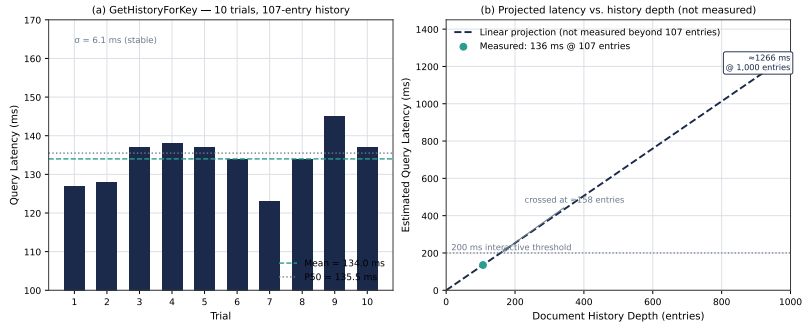
Figure 26: Experiment 7 Fabric GetHistoryForKey latency: 107-entry history depth measured directly; deeper data points are linear projections from this single measurement, not independently measured values. Multi-depth validation is future work.
