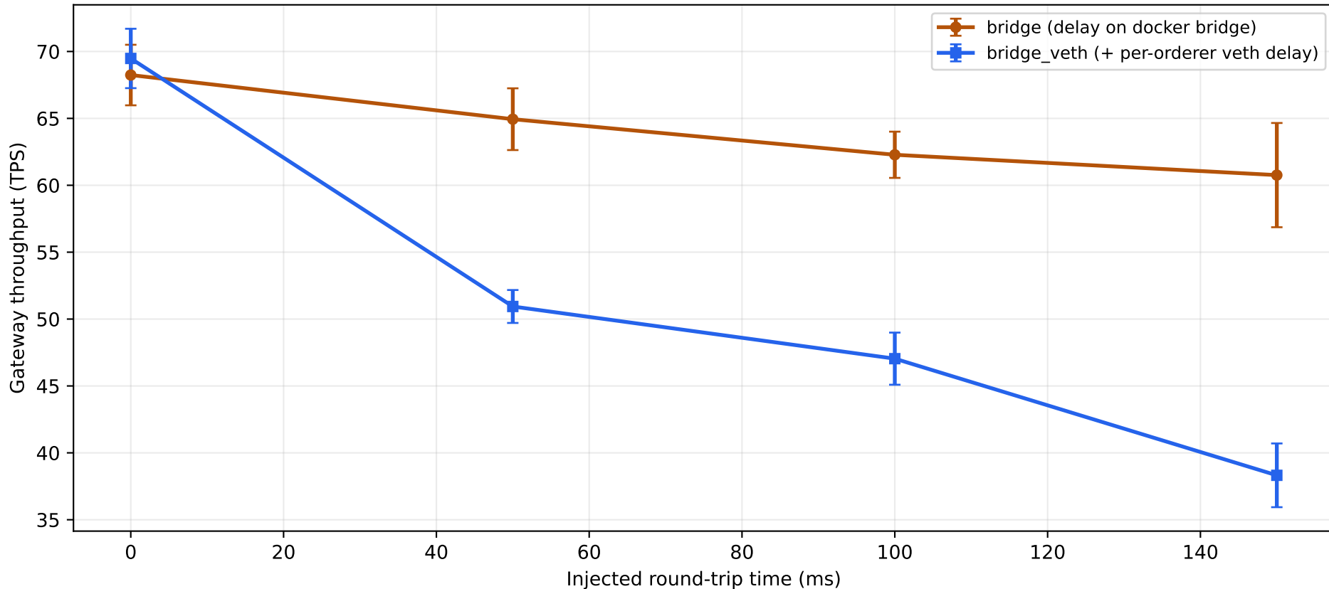
Exp 5 — WAN sensitivity (duration60s, conc 200, n=5/point), mean with 95% CI
