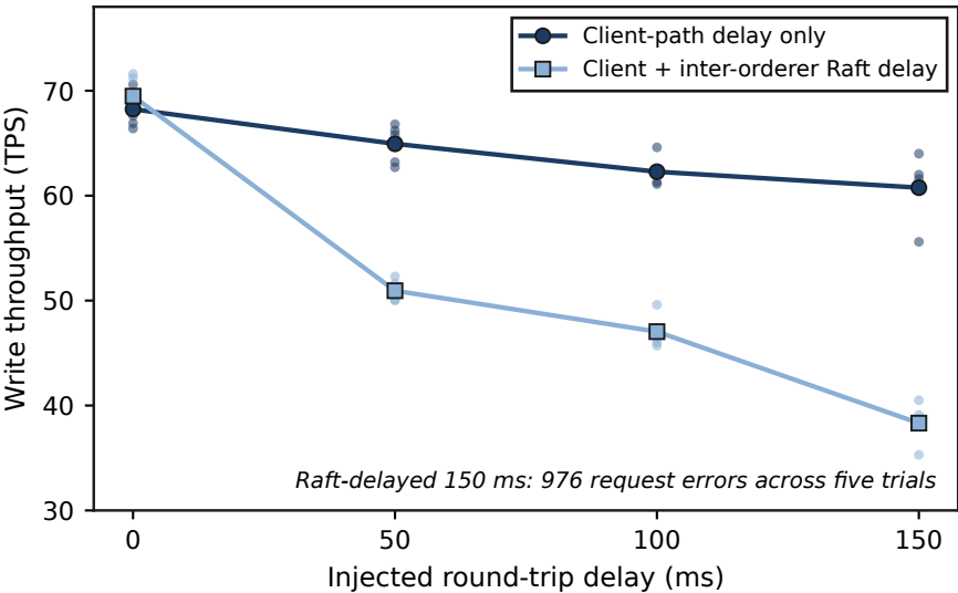
Throughput under injected WAN delay
