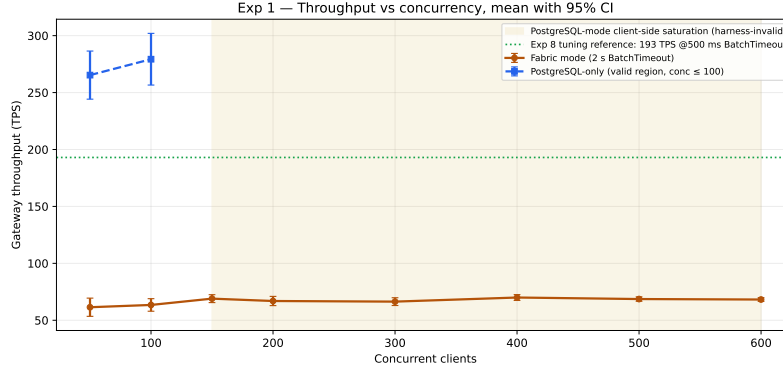
Figure 19: Experiment 1 scalability under concurrent load on Linux x86_64 (regenerated from released raw data; mean with 95 % t confidence intervals, n=5 per point): Fabric REST-gateway throughput compared with the PostgreSQL-only baseline restricted to its harness-valid region ( \text{conc} \leq 100 ); the shaded region marks PostgreSQL-mode client-side load-generator saturation (self-flagged invalid rows, excluded from analysis), and the dotted line is the Experiment 8 BatchTimeout tuning reference (193 TPS at 500 ms).
