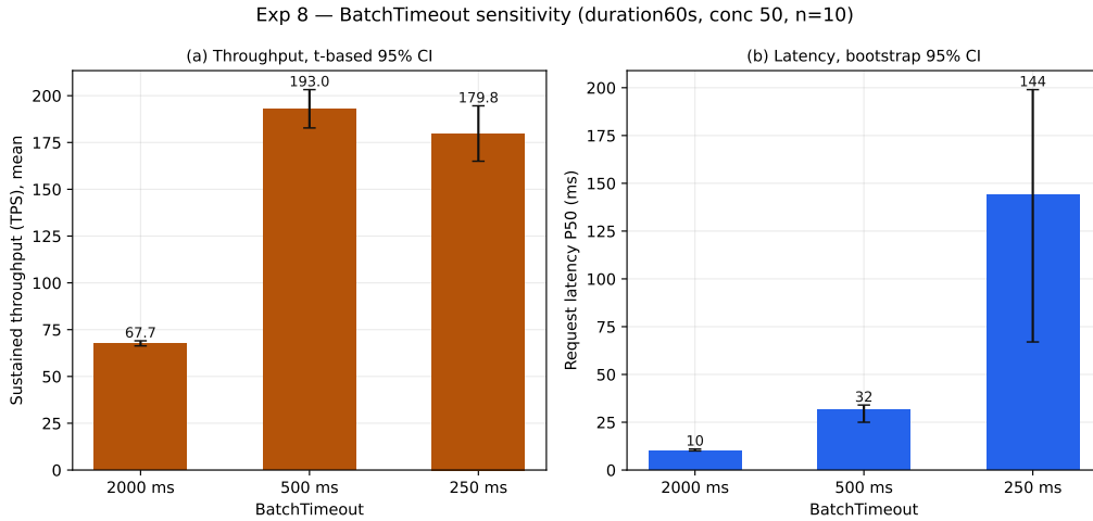
Figure 26: Experiment 8 BatchTimeout sensitivity (Linux x86_64, 50 clients; regenerated, n=10 per setting, zero-error runs): (a) sustained throughput (mean, t 95 % CI) and (b) request latency (P50, bootstrap 95 % CI) at 2 s, 500 ms, and 250 ms, showing the reproducible 500 ms optimum.
