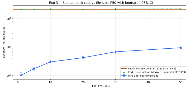
Figure 21: Experiment 3 file-size independence of ledger latency (Linux, direct Kubo API; regenerated with bootstrap 95 % CIs, n=10 per size): IPFS upload P50 (10–95 ms across 1–50 MB), the constant Fabric commit latency (2,132 ms band), and the derived end-to-end upload cost (commit + IPFS P50), matching the 2,142–2,226 ms range reported in the text.
