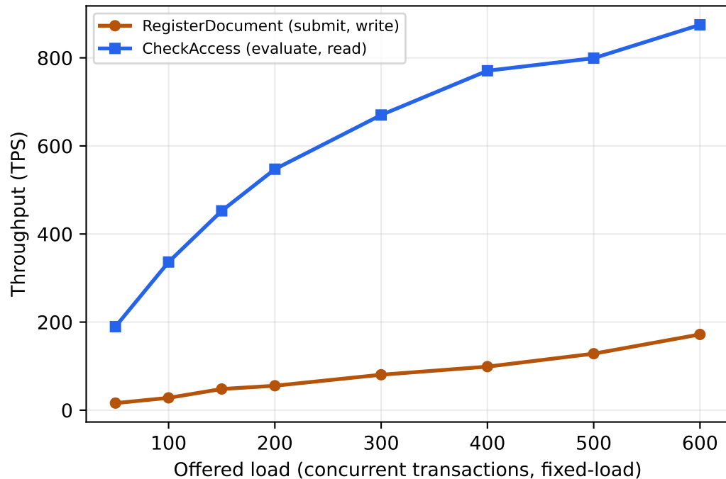
(a) Caliper throughput vs offered load
