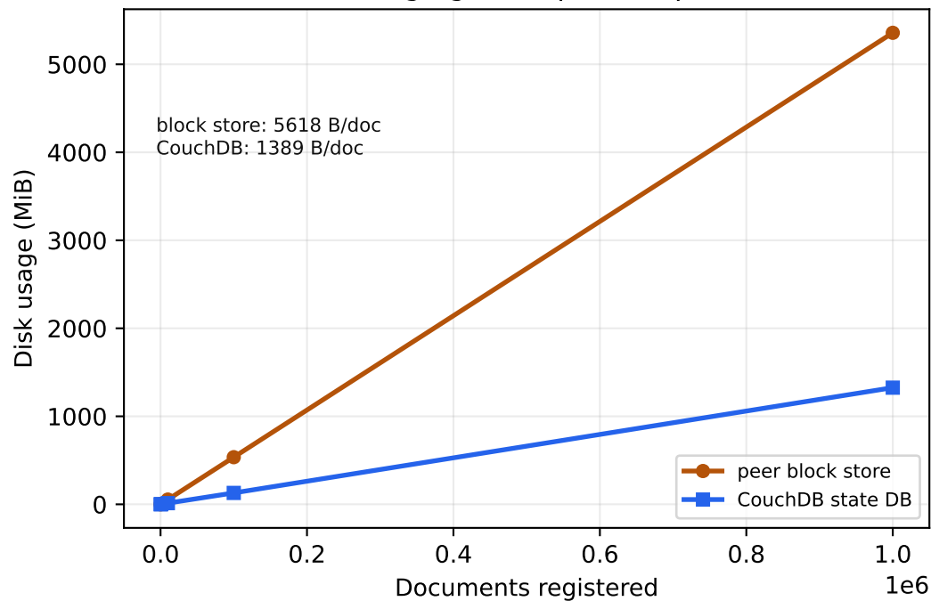
(b) Storage growth per component
