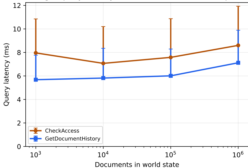
(a) Ledger query latency vs world-state size, P50 (caps: P95)
