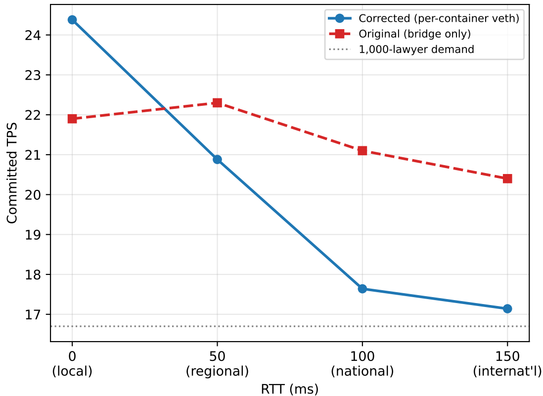
TPS vs RTT
