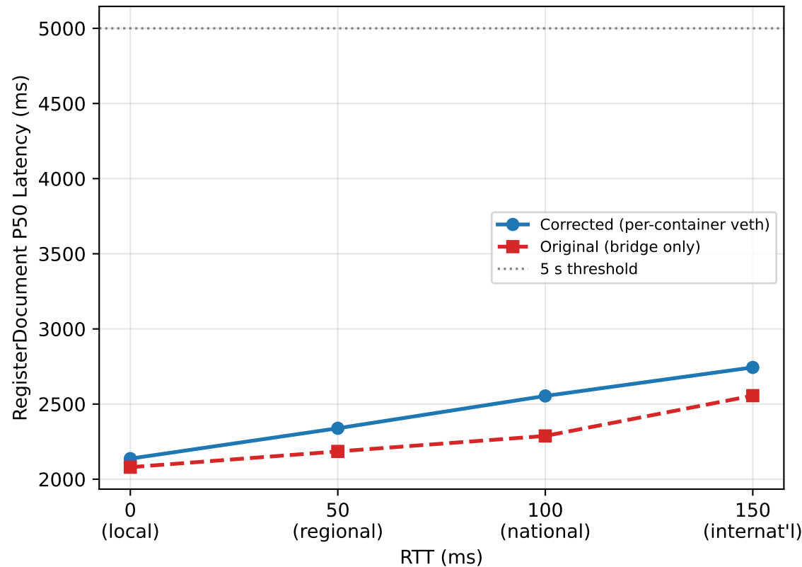
RegisterDocument P50 Latency vs RTT
