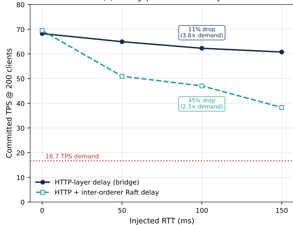
(a) Throughput vs. WAN latency
