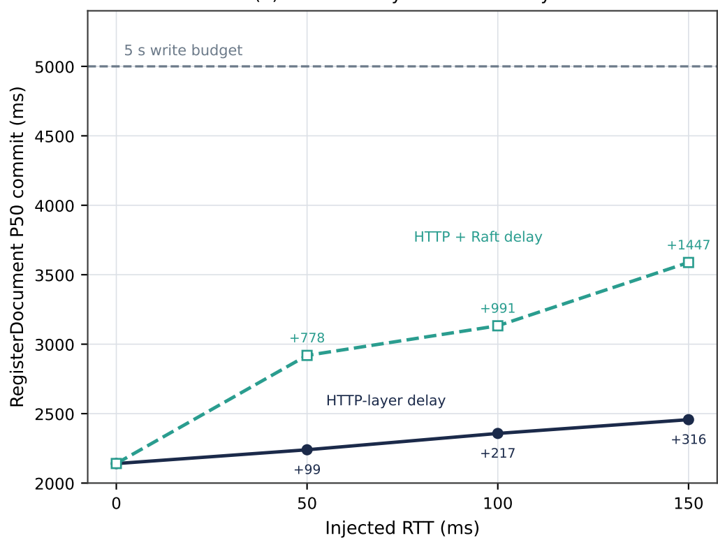
(b) Write latency vs. WAN latency
