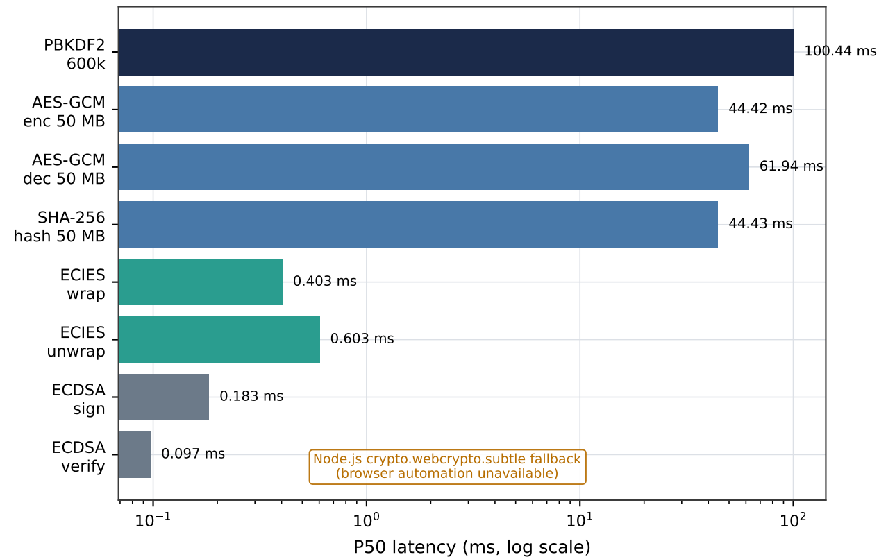
(a) Cryptographic operation costs
