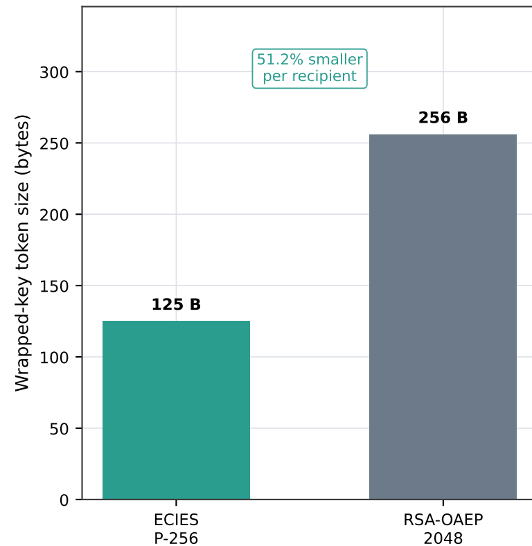
(b) Access-token storage cost
