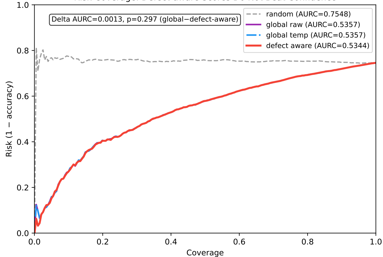
Risk-Coverage: Defect-aware Scores Do Not Beat Confidence
