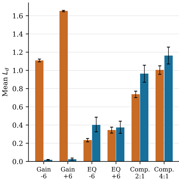
Audio distance
