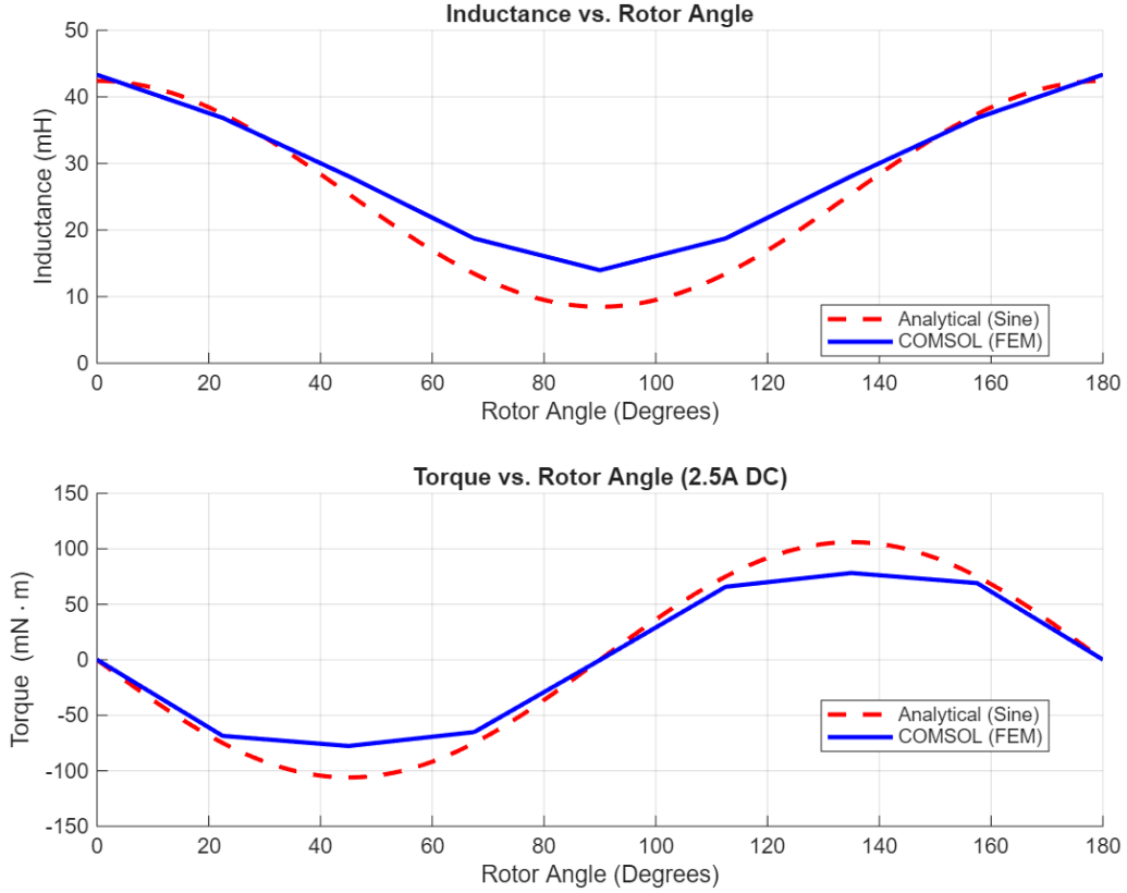
Figure 8: Comparison of analytical and non-linear FEM torque results.
