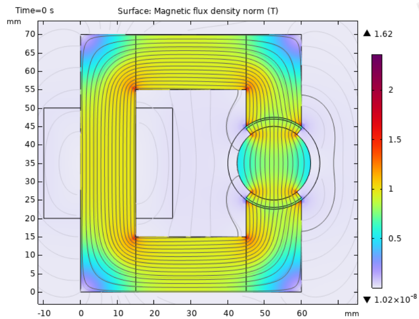
Figure 5: Flux density vectors at 0 degrees for non-linear soft iron.
