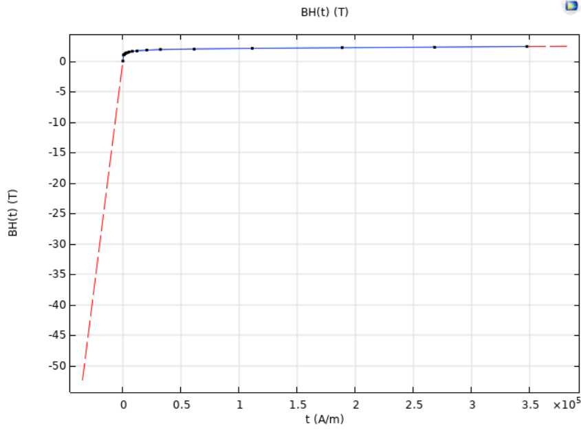
Figure 9: B-H magnetization curve for the Soft Iron core material.
