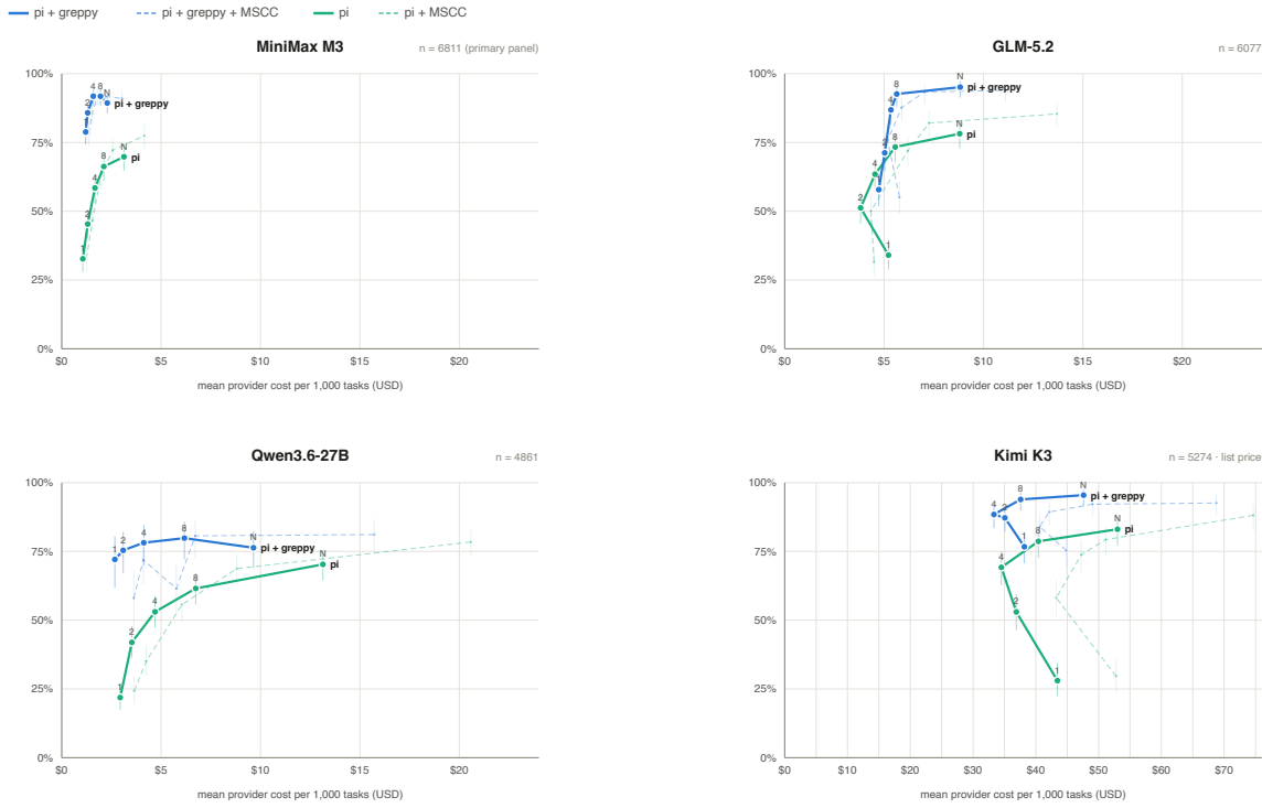
Navigation: success rate over real API cost per 1,000 tasks — four models
