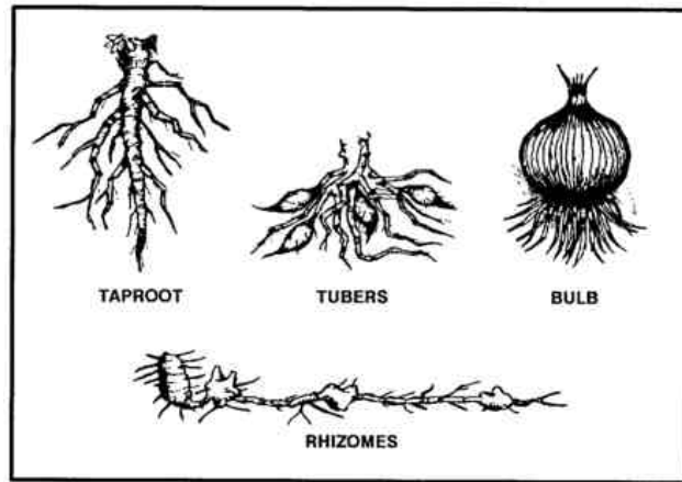
Figure 9-4. Root structures.
