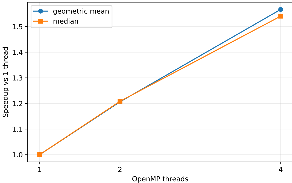
Refreshed evidence-layer scaling
