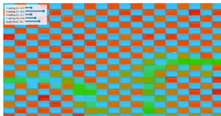
N,N-DMT Coupling Kernels Pattern
