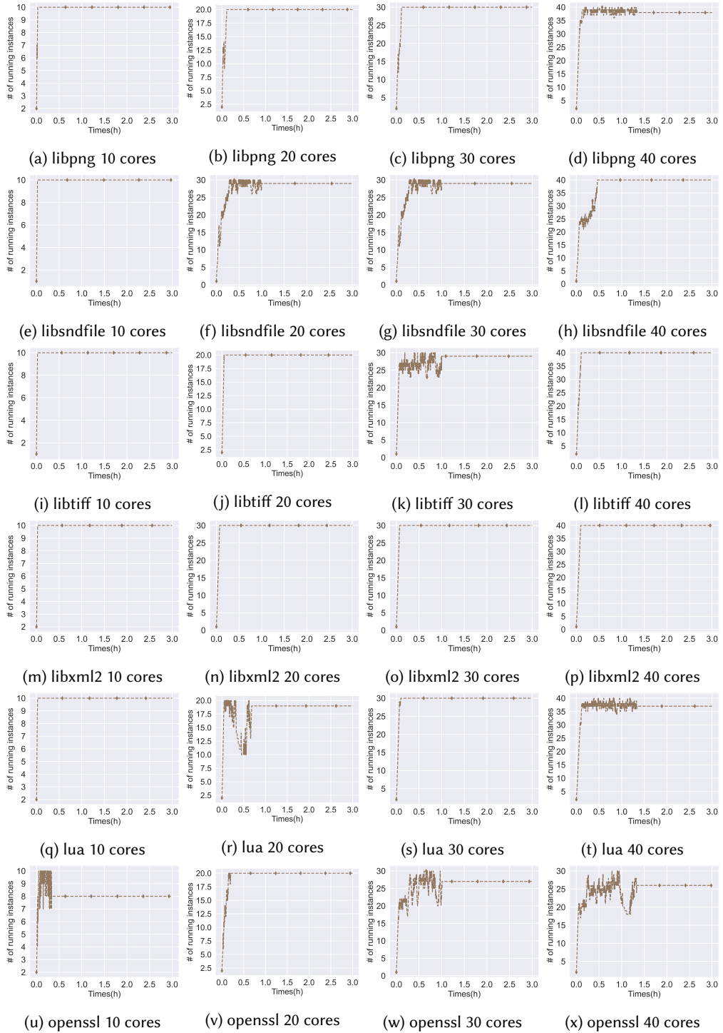
Fig. 1. The change in the number of running instances with time (3 hours) using 10, 20, 30 and 40 CPU cores.
