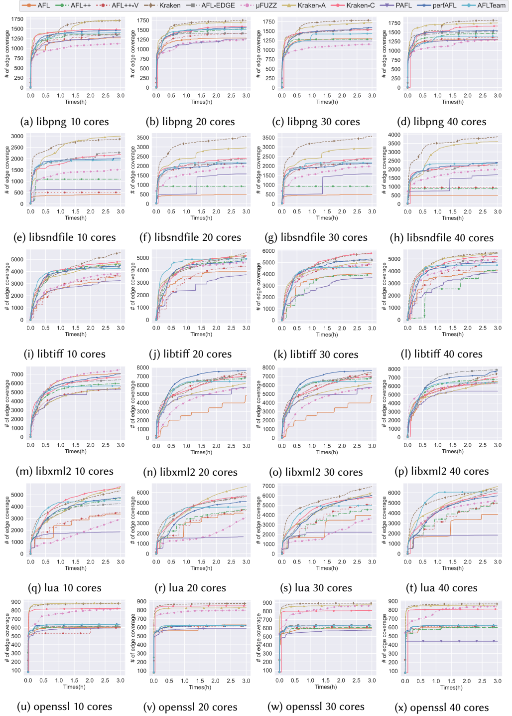
Fig. 3. Edge coverage changes with time (3 hours) using 10, 20, 30 and 40 CPU cores.
