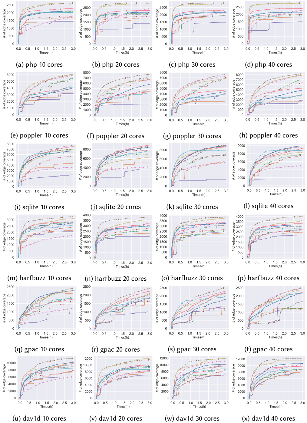
Fig. 4. Edge coverage changes with time (3 hours) using 10, 20, 30 and 40 CPU cores (Cont.).
