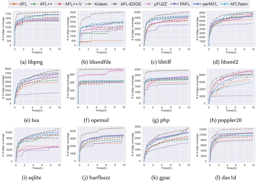
Fig. 5. Edge coverage changes in 10 hours using 20 cores.
