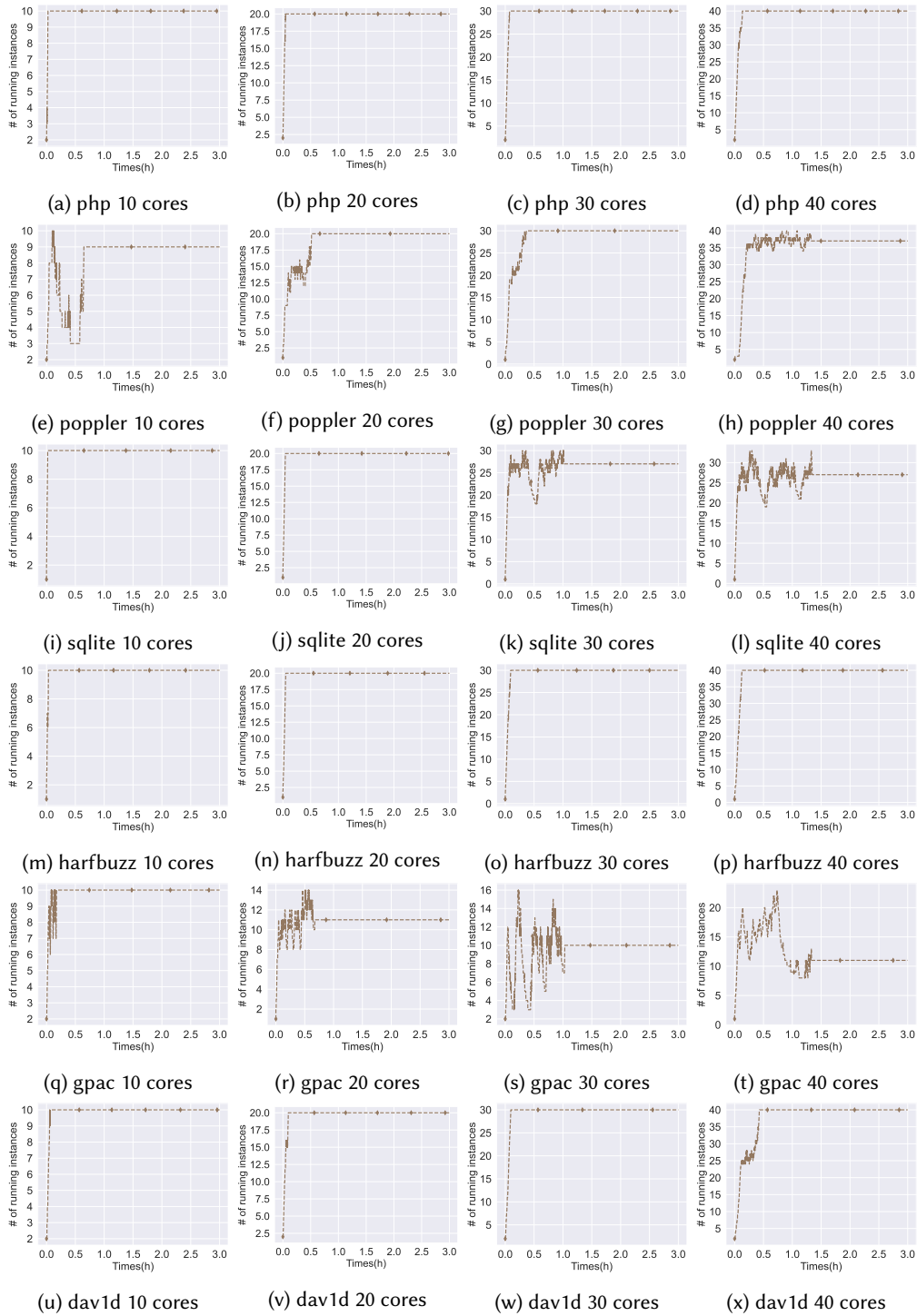
Fig. 2. The change in the number of running instances with time (3 hours) using 10, 20, 30 and 40 CPU cores (Cont.).
