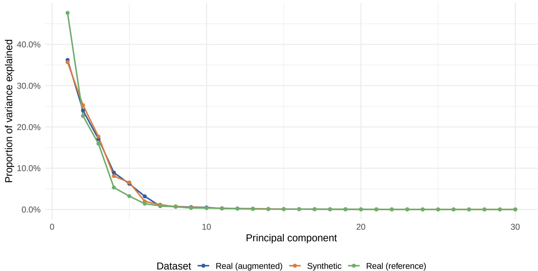
Scree plot: variance explained by the first 30 principal components
