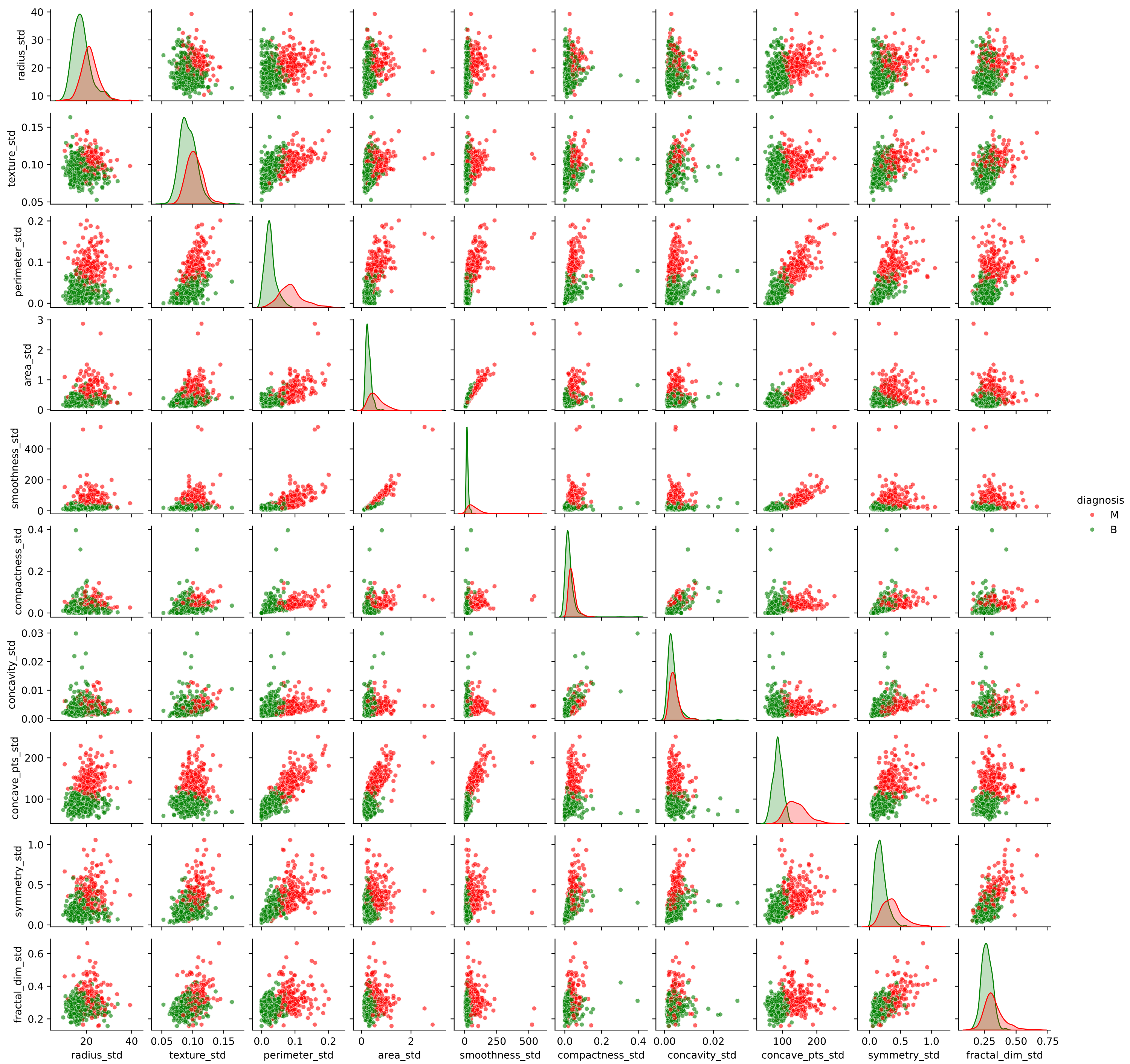
Pairwise Scatterplots of features
