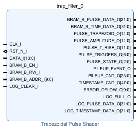
Figure 4.2. Top level interface of Trapezoidal Pulse Shaper IP Core found in the Vivado block design window.
