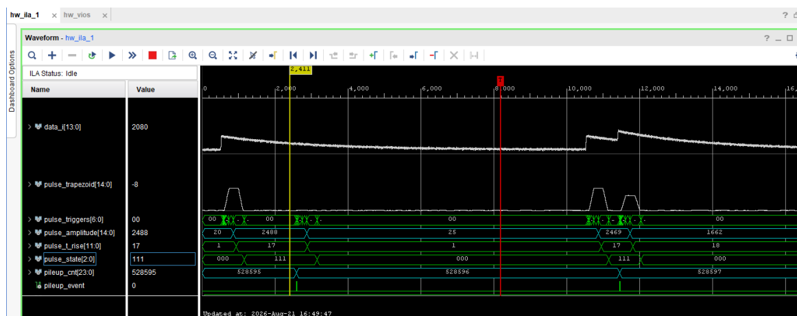
Figure 6.5. ILA waveform for the pulse stimulus in the ZedBoard. First two pulses are valid while the third event is affected by pileup.
