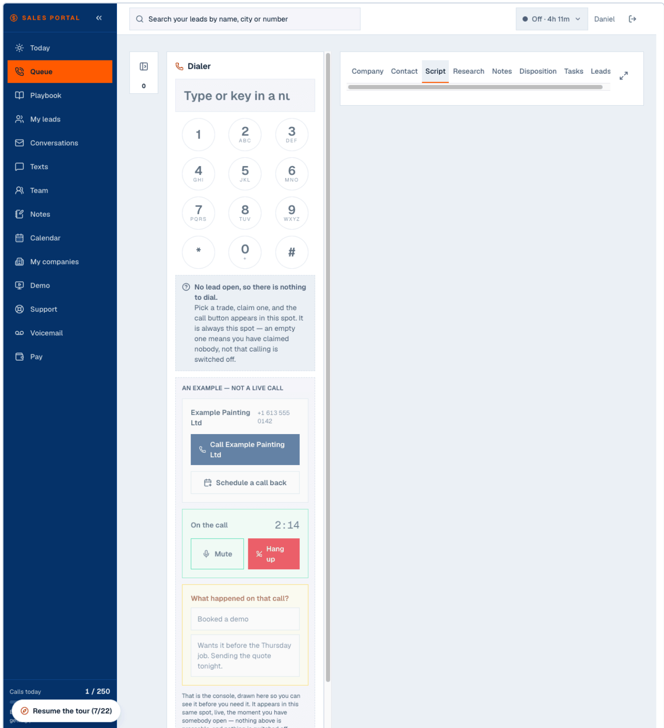
Figure 4 — The console at rest: sidebar, top bar with the status menu, the Dialer on the left, the tabbed card on the right with Script open.
