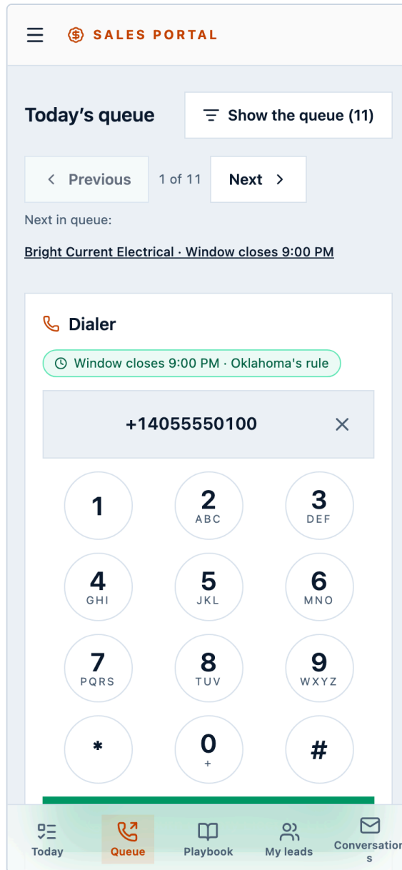
Figure 14 — The console on a phone: dialer first, the queue as a drawer.
