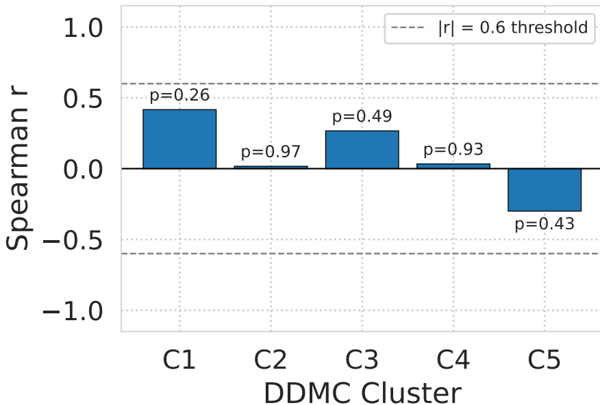
Panel B — AXL Abundance vs. Cluster Centers (KO excluded)
