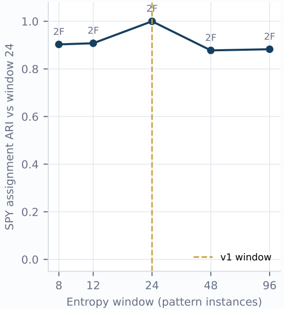
C Downstream entropy sensitivity
