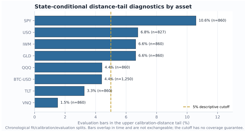
Figure 4: Asset heterogeneity in the empirical distance-tail diagnostic. The dashed line is a descriptive cutoff, not a promised coverage level.
