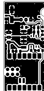
TOP COPPER
