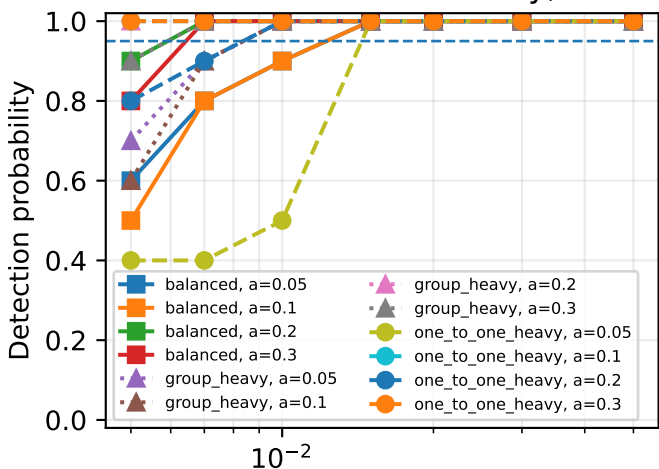
Interactivity structure sensitivity, N=12000
