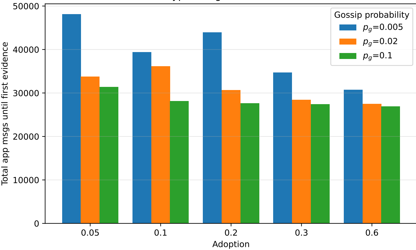
Typical regime, N=12000
