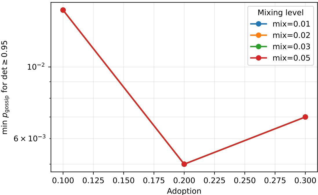
Mixing threshold summary, N=12000
